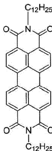
Comparative Compound c2
