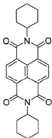
Comparative Compound c1
