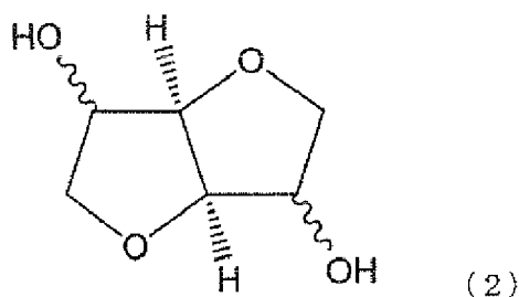
[Chem. 8]
