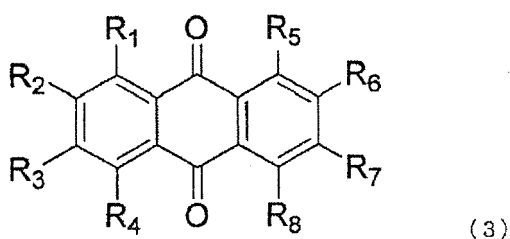
[Chem. 4]
