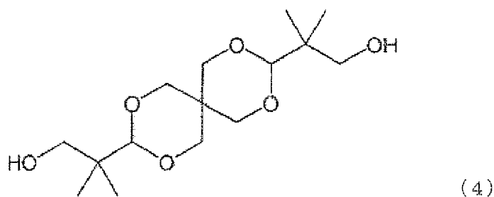
[Chem. 9]
