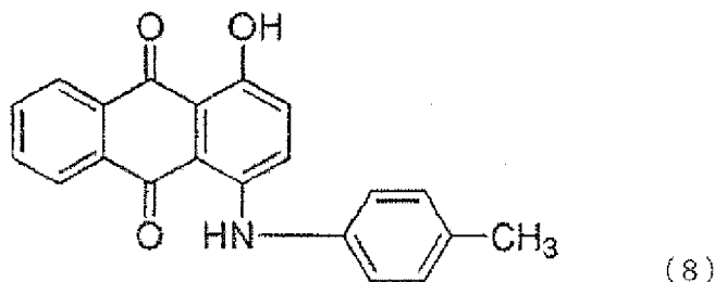
[Chem. 14]
