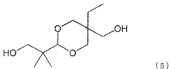
[Chem. 10]
