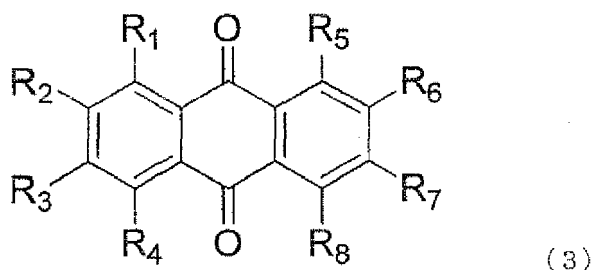
[Chem. 4]
