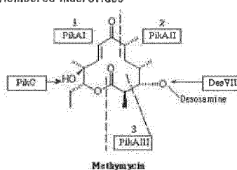
12-Membered macrolides
