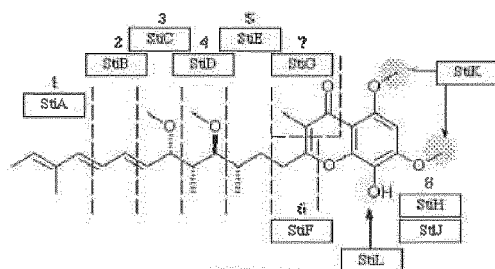
Stigmatellin A
