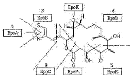
Epothikone A
