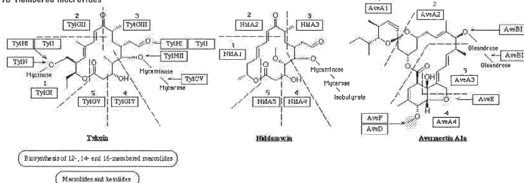
16-Membered macrolides
