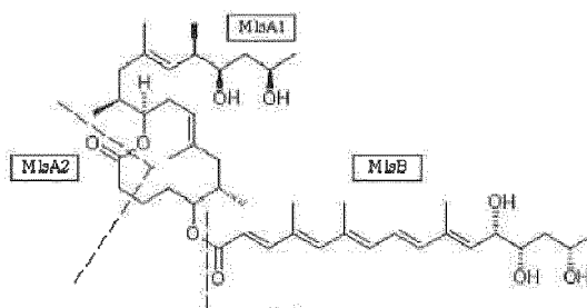
Mycolactone
