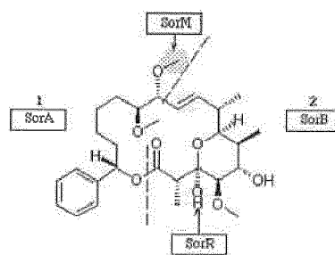
Soraphen A
