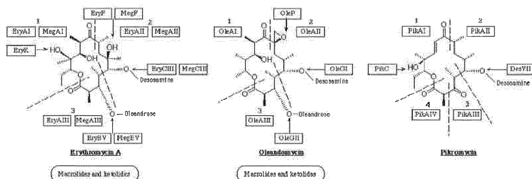
14-Membered macrolides
