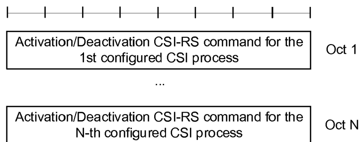
A) Activation/Deactivation of CSI-RS resources MAC Control Element
