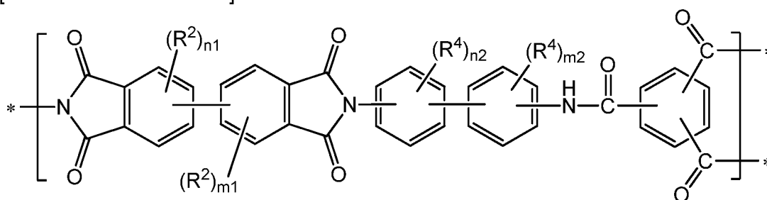
[Chemical Formula 1-3]
