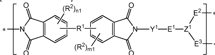
[Chemical Formula 1]
