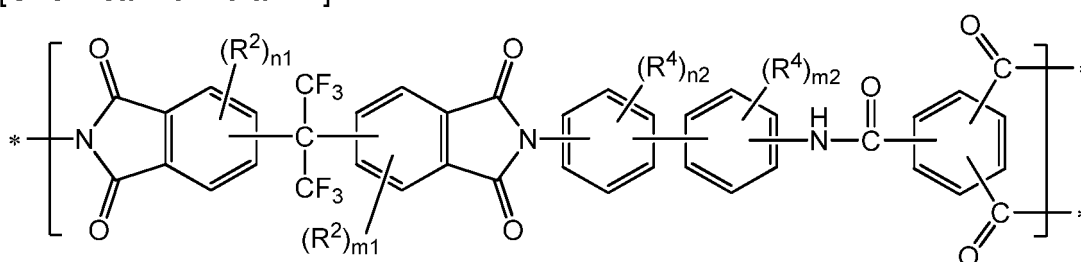
[Chemical Formula 1-2]
