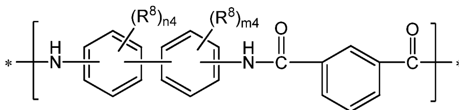
[Chemical Formula 3-2]
