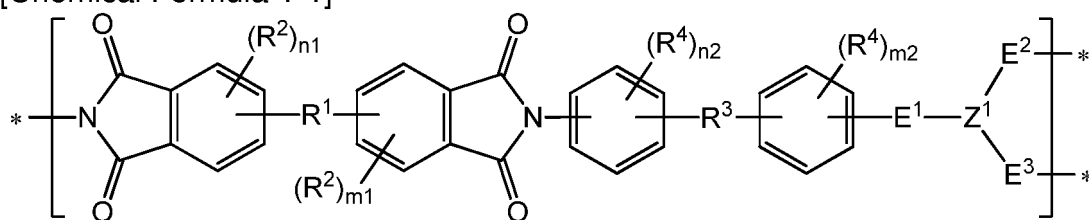
[Chemical Formula 1-1]
