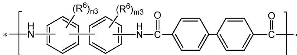
[Chemical Formula 2-3]
