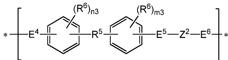
[Chemical Formula 2-1]
