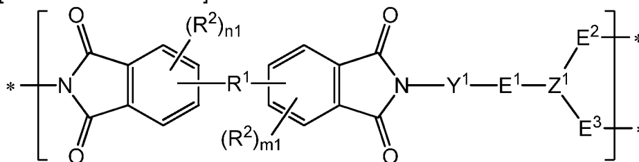
[Chemical Formula 1]
