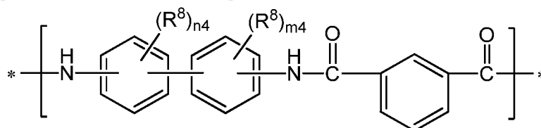
[Chemical Formula 3-2]
