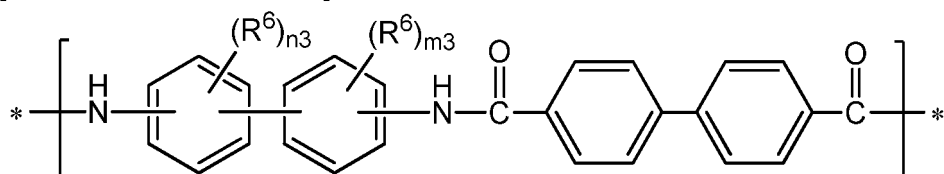
[Chemical Formula 2-3]
