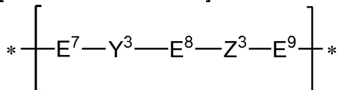
[Chemical Formula 3]
