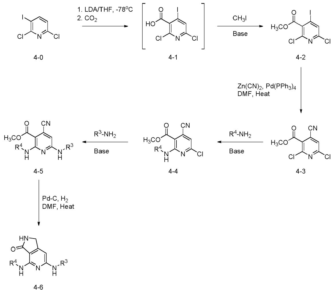
Scheme 4
