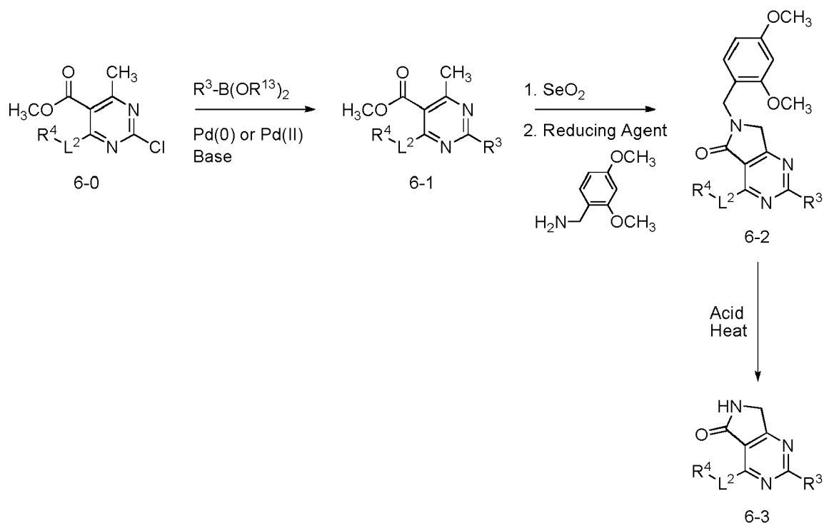
Scheme 6
