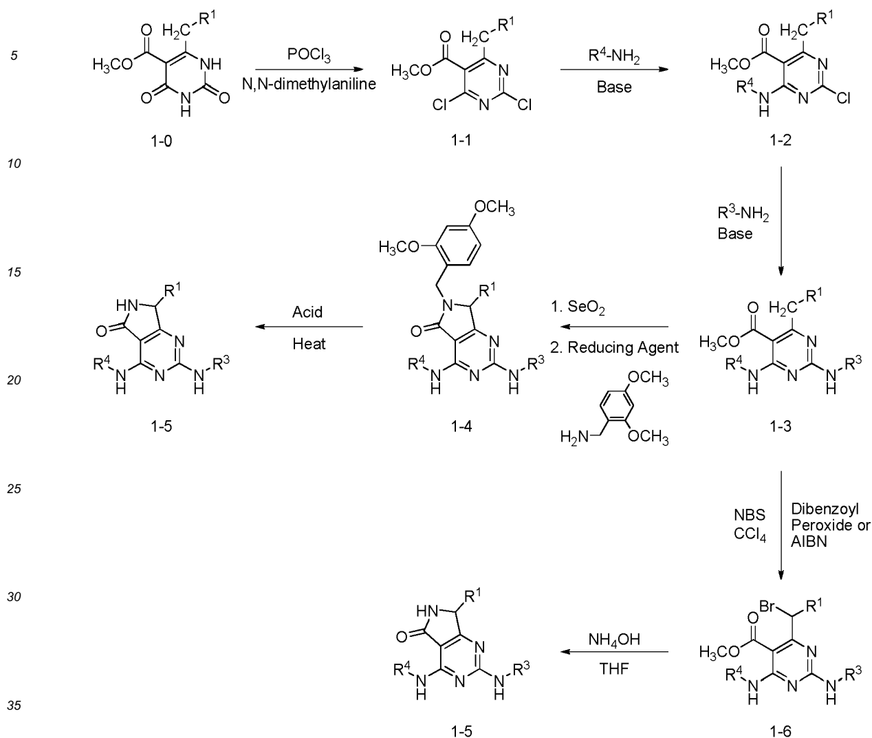
Scheme 1
