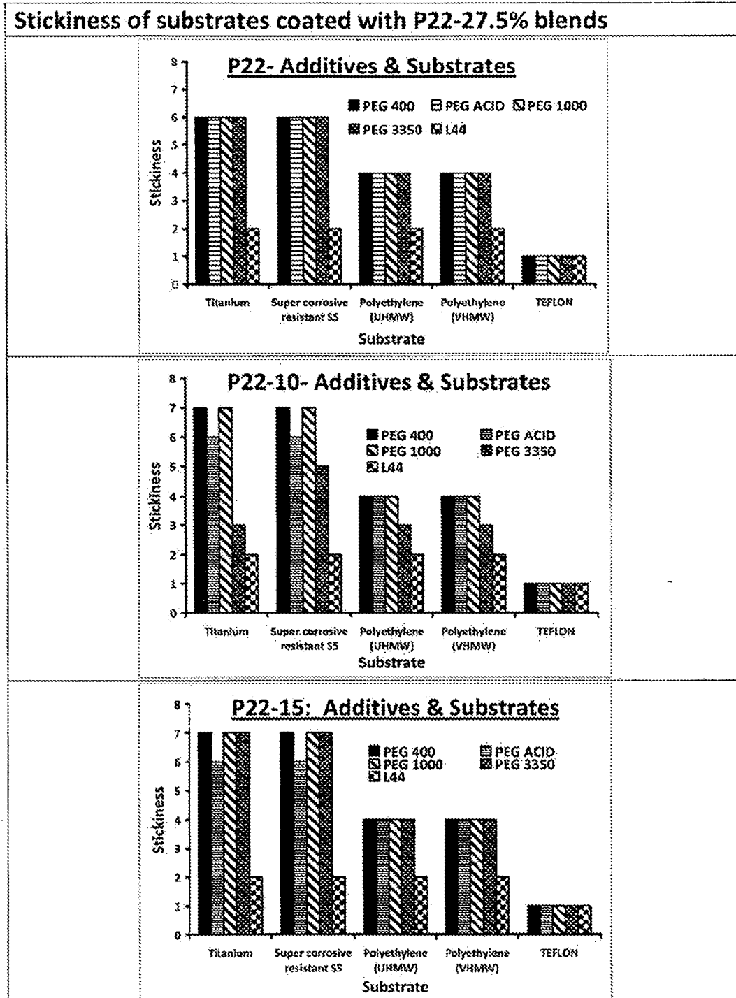
FIG. 6 Stickiness of substrates coated with P22-27.5% Blends of PEGS
