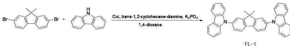
[Reaction Formula 1]
