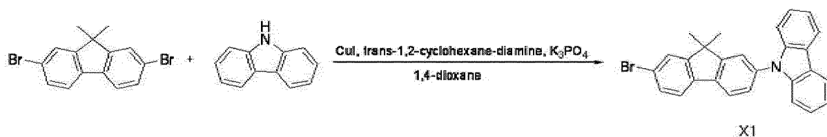
[Reaction Formula 2]
