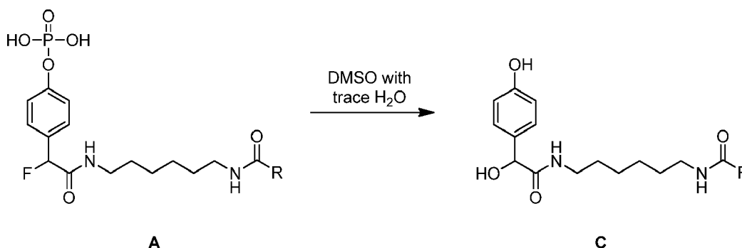
Scheme 15
