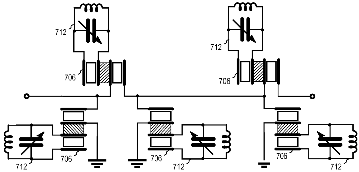
2 ½ order variant of filter of Figure 10C
