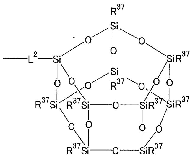
[Chem. 22]
