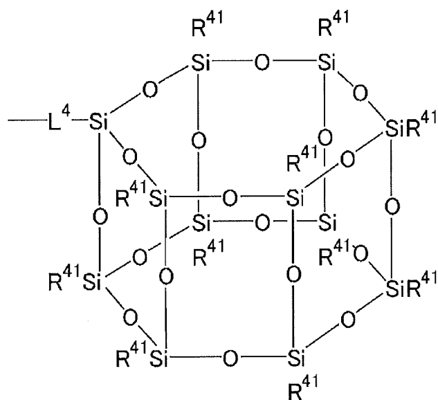
[Chem. 36]
