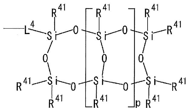
[Chem. 37]
