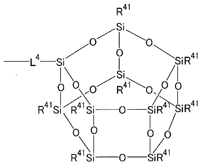
[Chem. 36]
