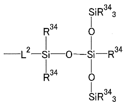
[Chem. 12]
