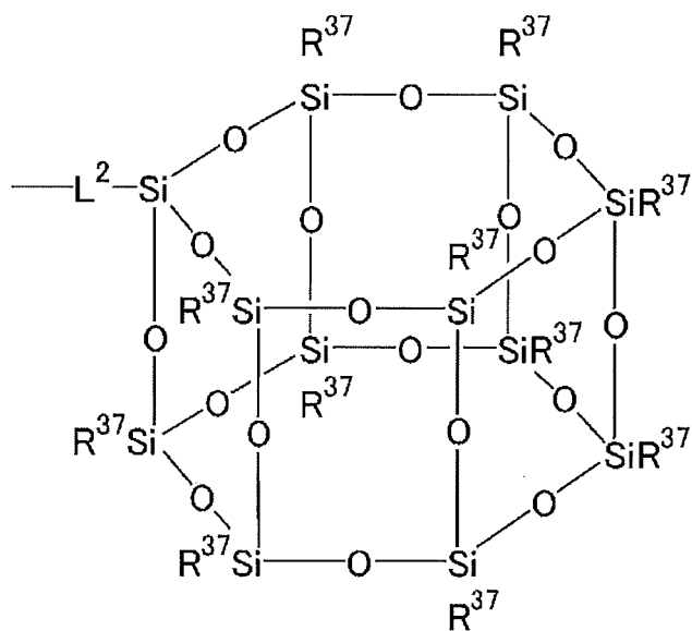
[Chem. 22]
