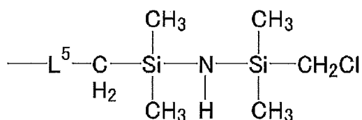
[Chem. 42]
