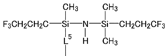
[Chem. 43]
