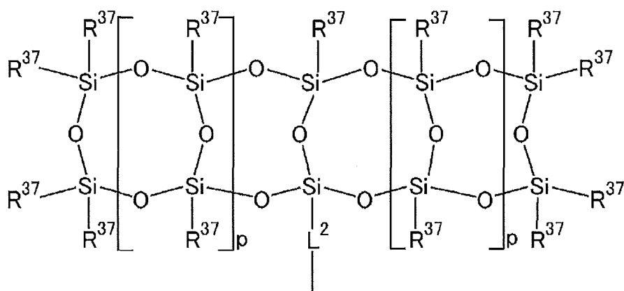
[Chem. 24]
