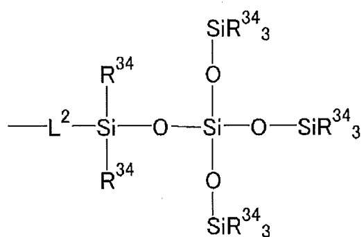
[Chem. 13]
