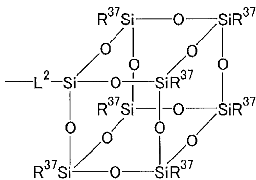
[Chem. 20]
