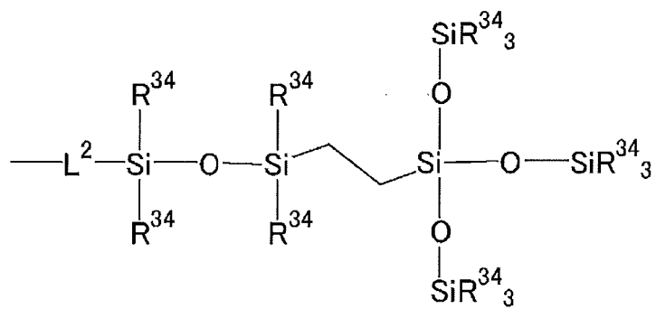
[Chem. 14]
