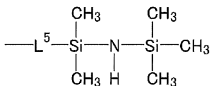
[Chem. 41]
