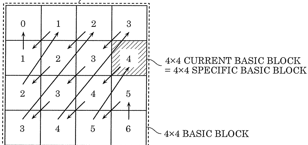
FIG. 21 THE NUMBER OF NON-ZERO COEFFICIENTS IN PRECEDING BASIC BLOCK
