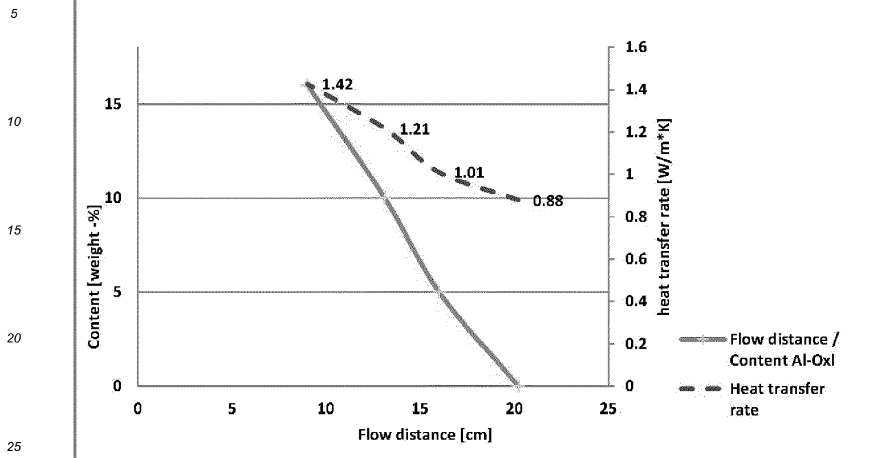
Graph 1: Average results of heat transfer and flow distance
