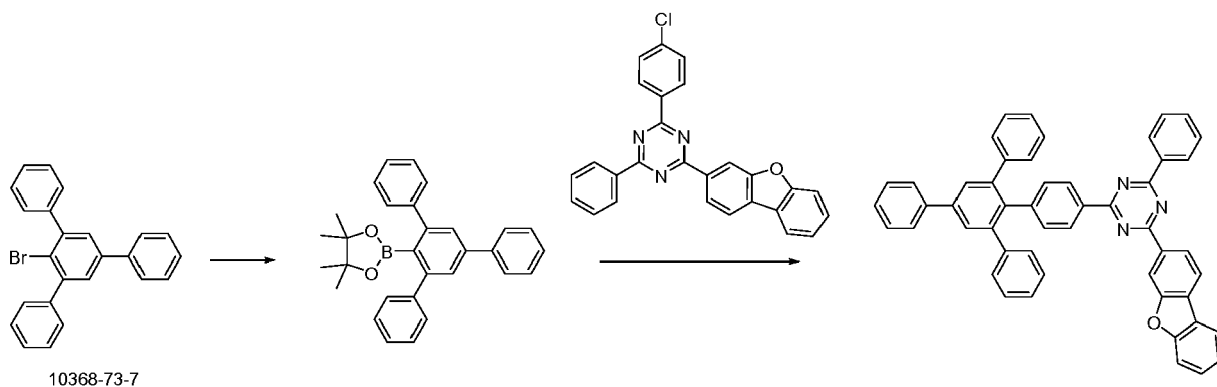
4,4,5,5-tetramethyl-2-(5'-phenyl-[1,1':3',1''-terphenyl]-2'-yl)-1,3,2-dioxaborolane
