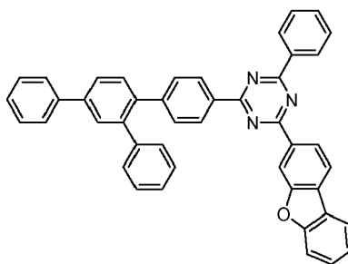
2-(dibenzo[b,d]furan-3-yl)-4-phenyl-6-(4'-phenyl-[1,1':2',1''-terphenyl]-4-yl)-1,3,5-triazine
