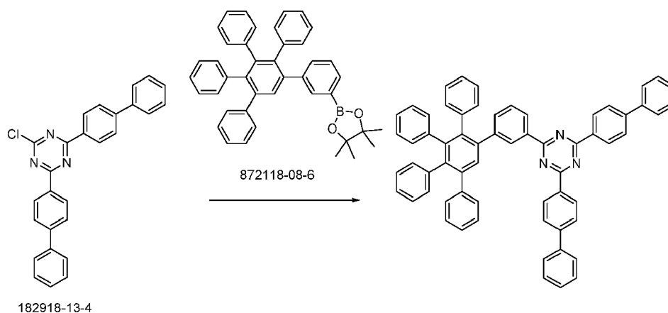
2,4-di([1,1'-biphenyl]-4-yl)-6-(3',4',5'-triphenyl-[1,1':2',1''-terphenyl]-4-yl)-1,3,5-triazine
