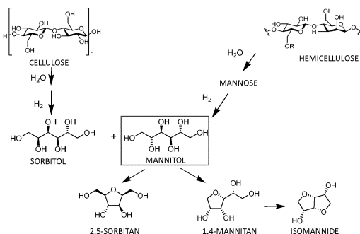
Fig. 1 REACTION OF CONVERSION FROM CELLULOSE OR HEMICELLULOSE INTO ISOMANNIDE OR 2,5-SORBITAN
