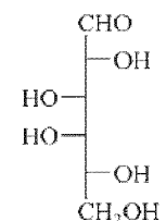
D-Galactose (D-Gal)
