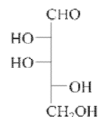
D-Lyxose (D-Lyx)
