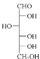
D-Glucose (D-Glu)
