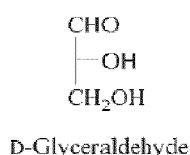
D-Glyceraldehyde
