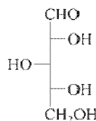
D-Xylose (D-Xyl)
