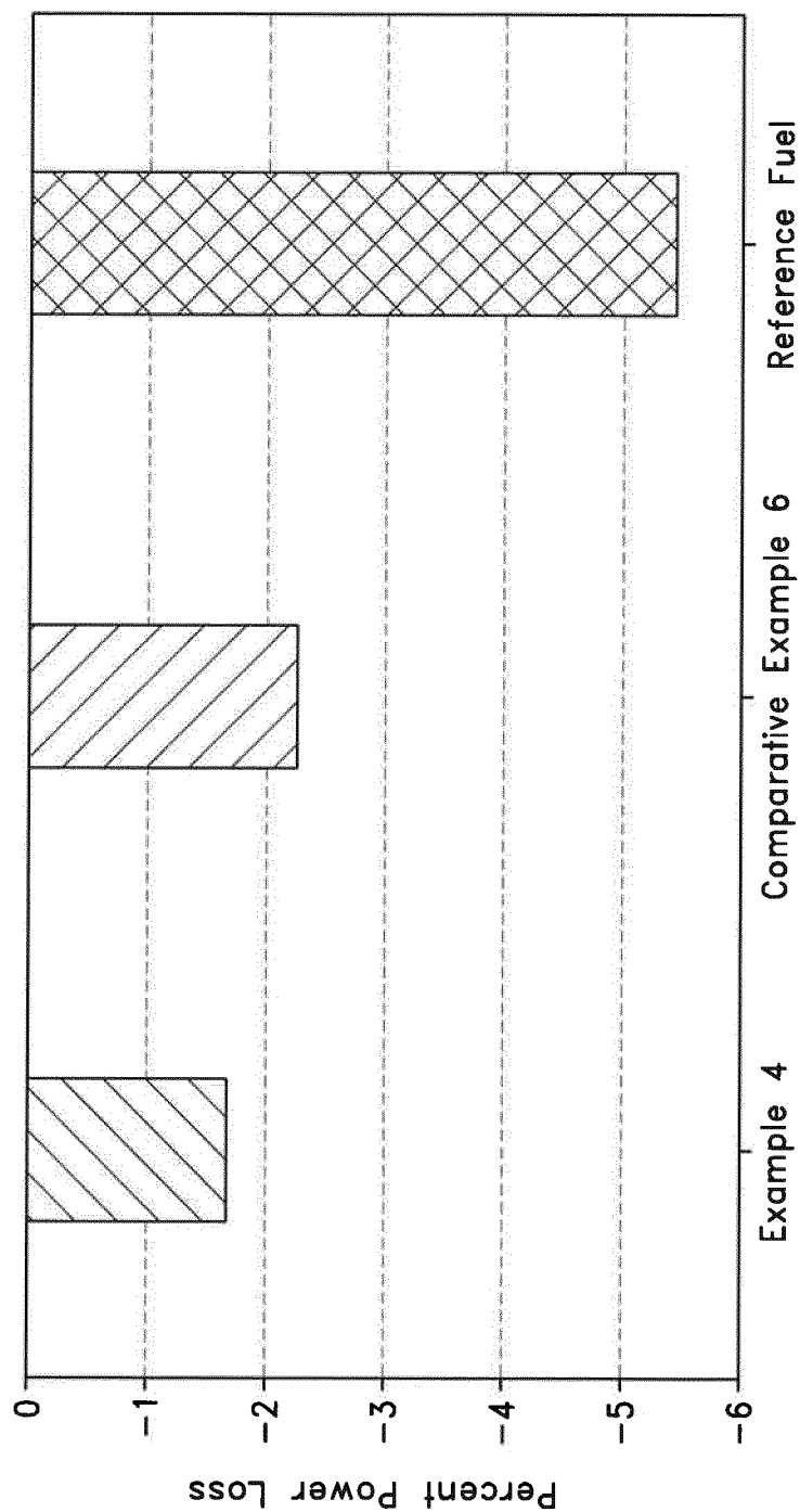
CEC F-98-08 DW10B Test Results
