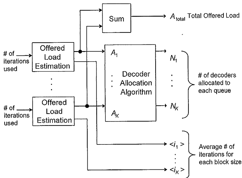
N_{dec} decoders to be allocated to K Queues
