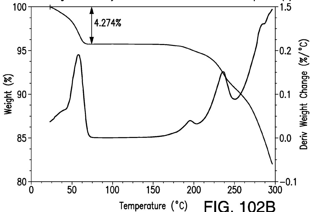
TGA Thermogram of a Hydrate of HCl Salt of Racemic Compound (I)
