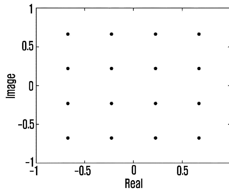
(b) PC2: SFBC(16QAM) / Rank1(16QAM)
