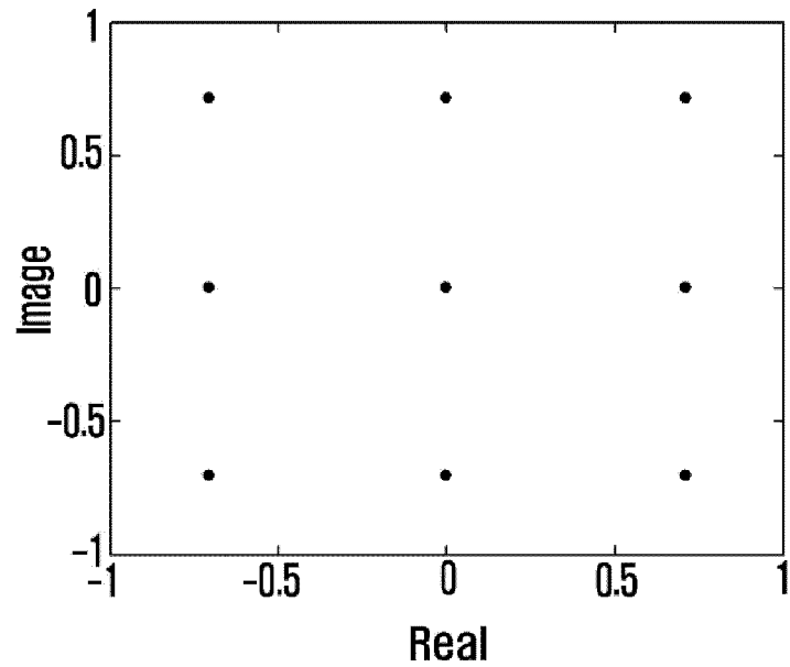
(c) PC3: Rank2(QPSK+QPSK)
