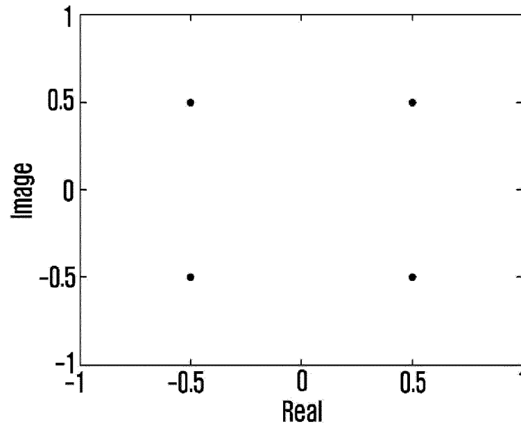
(a) PC1: SFBC(QPSK) / Rank1(QPSK)
