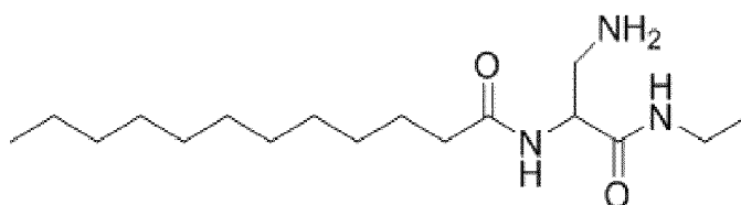
N-[2-amino-1-(ethylcarbamoyl)ethyl]dodecanamide
