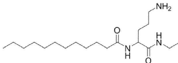
N-[4-amino-1-(ethylcarbamoyl)butyl]dodecanamide
