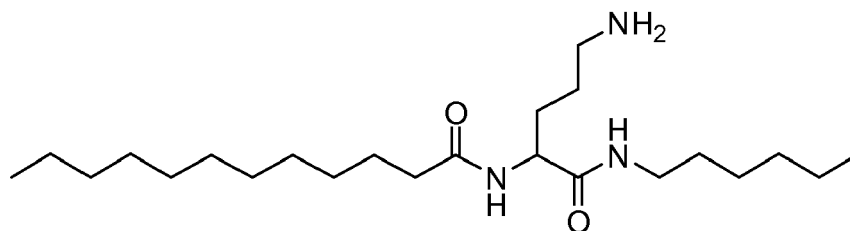
N-(5-amino-1-(hexylamino)-1-oxopentan-2-yl)dodecanamide
