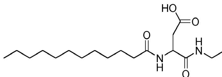
3-dodecanamido-4-(ethylamino)-4-oxobutanoic acid
