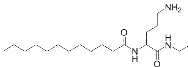
N-[4-amino-1-(ethylcarbamoyl)butyl]dodecanamide
