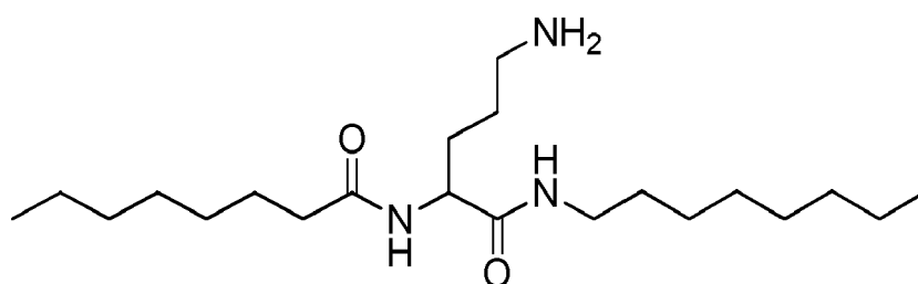
N -(5-amino-1-(octylamino)-1-oxopentan-2-yl)octanamide
