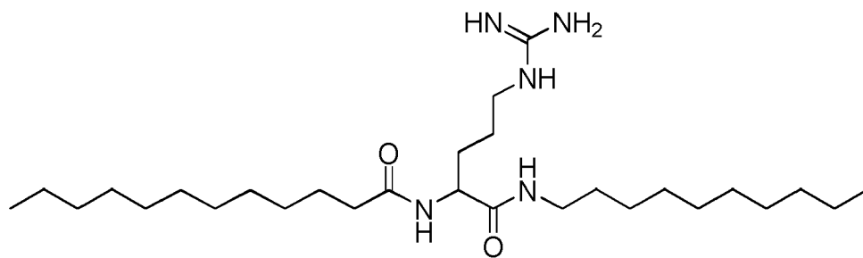
N -(1-(decylamino)-5-guanidino-1-oxopentan-2-yl)dodecanamide
