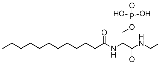
2-dodecanamido-3-(ethylamino)-3-oxopropyl dihydrogen phosphate
