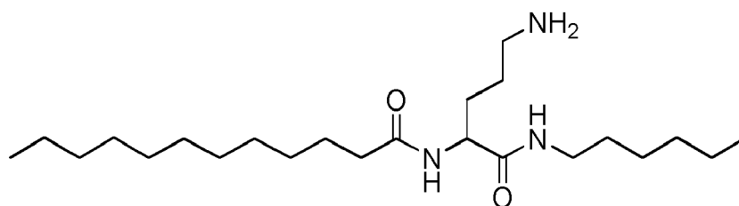
N -(5-amino-1-(hexylamino)-1-oxopentan-2-yl)dodecanamide
