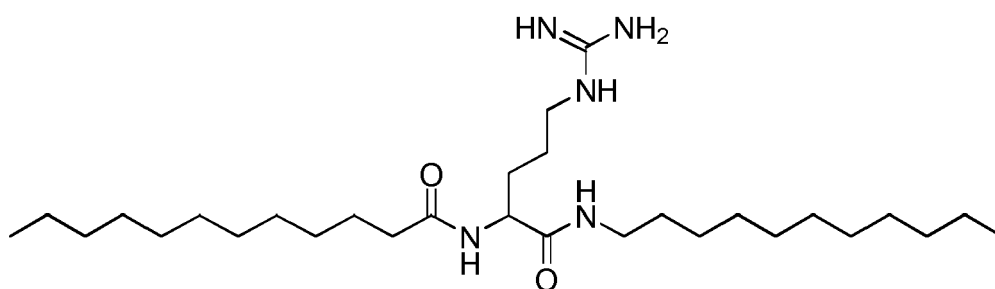
N -(5-guanidino-1-oxo-1-(undecylamino)pentan-2-yl)dodecanamide
