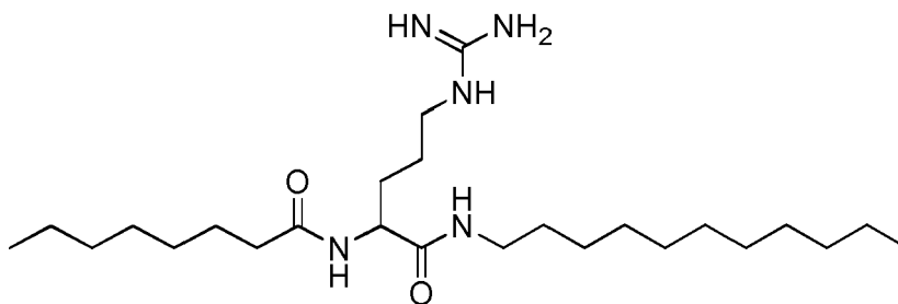
N -(5-guanidino-1-oxo-1-(undecylamino)pentan-2-yl)octanamide
