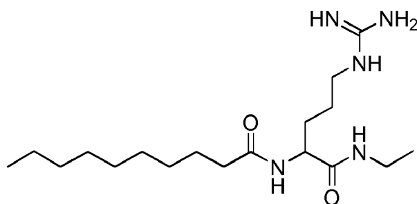
N -(1-(ethylamino)-5-guanidino-1-oxopentan-2-yl)decanamide
