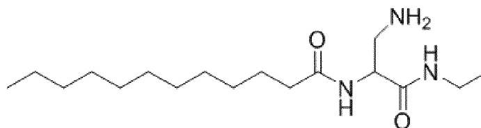
N-[2-amino-1-(ethylcarbamoyl)ethyl]dodecanamide
