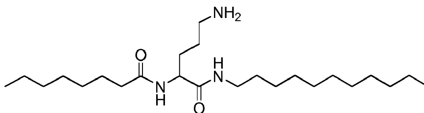
N -(5-amino-1-oxo-1-(undecylamino)pentan-2-yl)octanamide
