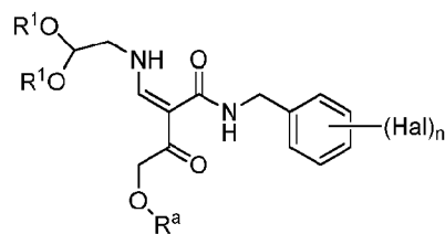
(E-1) (Z)-configuration
