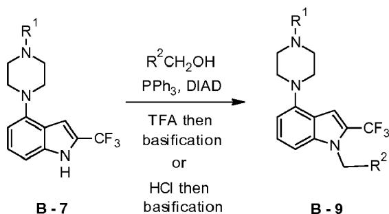
Reaction Scheme 6.
