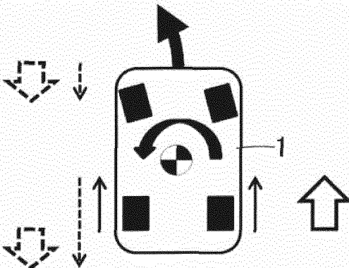
Fig. 13C CASE OF REAR-WHEEL DRIVE VEHICLE (YAW MOMENT CONTROL BY FRICTION BRAKE) → DRIVING TORQUE (ENGINE OUTPUT) --- BRAKING TORQUE (FRICTION BRAKE)
