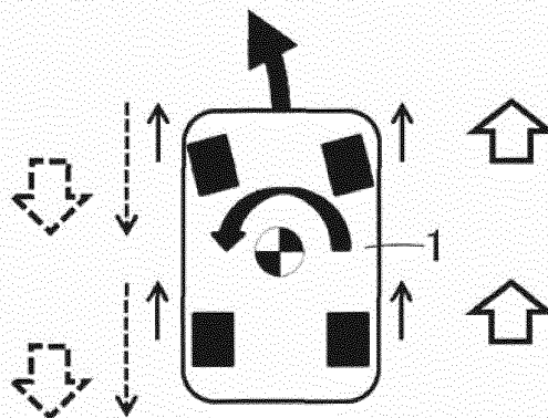
Fig. 13B CASE OF FRONT-WHEEL DRIVE VEHICLE (YAW MOMENT CONTROL BY FRICTION BRAKE) → DRIVING TORQUE (ENGINE OUTPUT) --- BRAKING TORQUE (FRICTION BRAKE)
