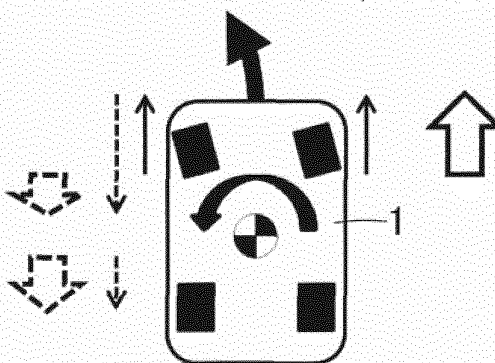
Fig. 13B CASE OF FRONT-WHEEL DRIVE VEHICLE (YAW MOMENT CONTROL BY FRICTION BRAKE) → DRIVING TORQUE (ENGINE OUTPUT) --- BRAKING TORQUE (FRICTION BRAKE)
