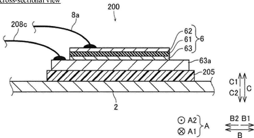
FIG. 5 600-600 cross-sectional view
