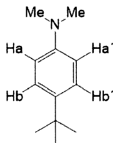
tBDA
