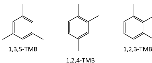
TMB isomers
