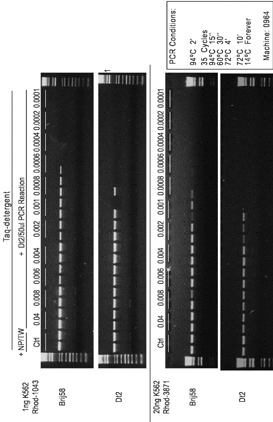
FIGURE 5 PCR Activity: Comparison of Brij58 alone to Dt2
