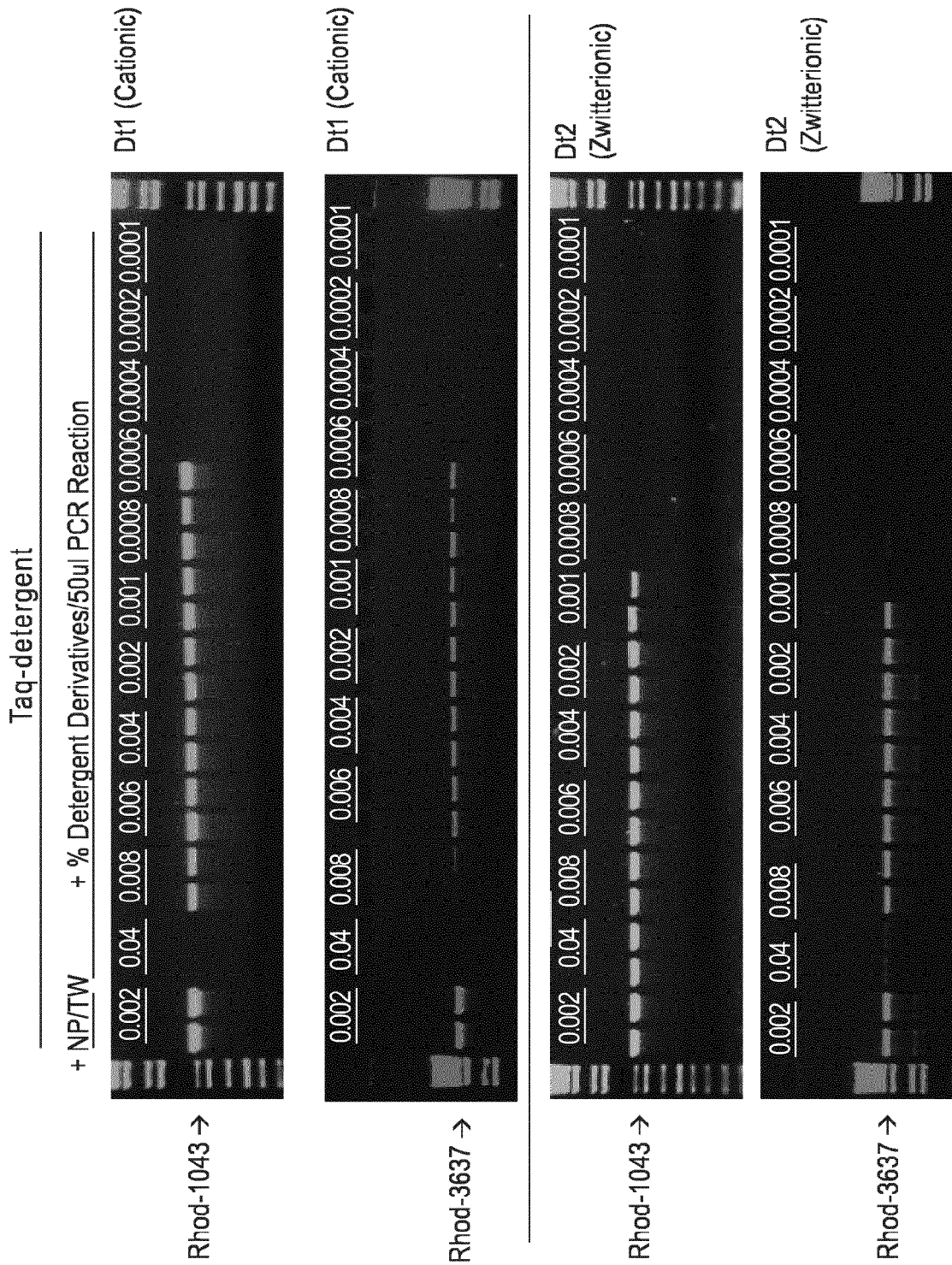
FIGURE 1 Titration of Dt1 and Dt2 at 11 different concentrations using 1Kb and 3Kb PCR products
