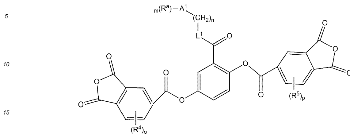
Chemical Formula 14-2
