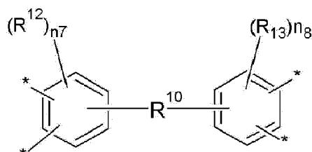
Chemical Formula 4
