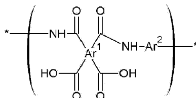
Chemical Formula 2
