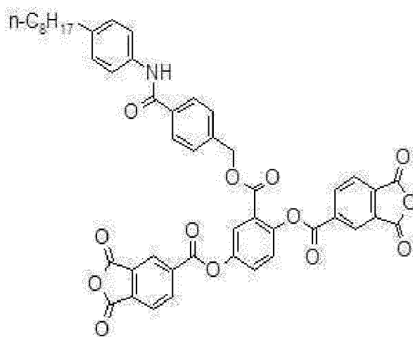
Compound M-17
