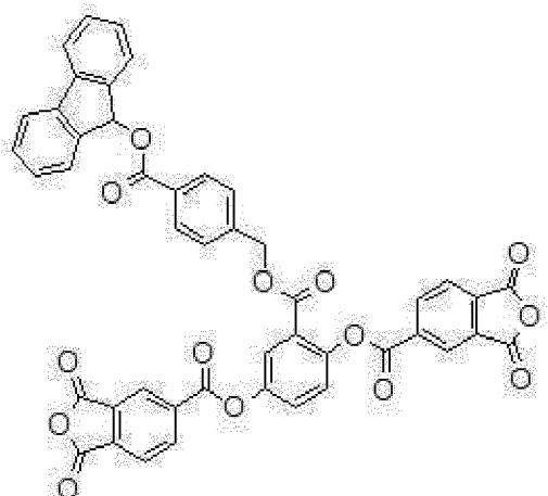
Compound M-14
