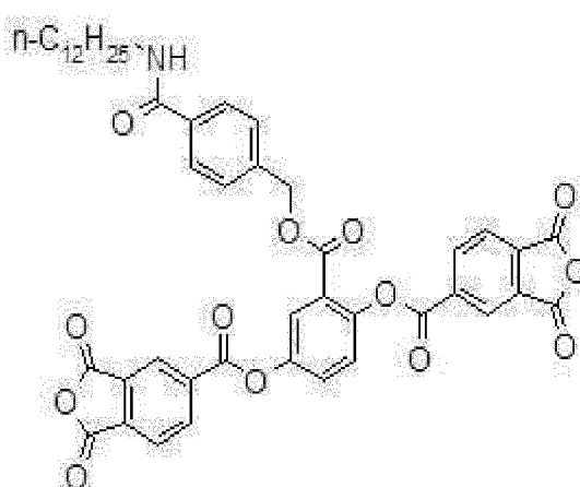
Compound M-15
