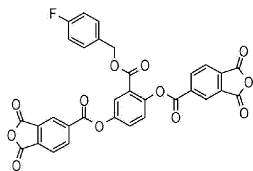
Compound M-5
