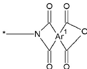
Chemical Formula 8
