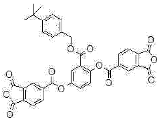
Compound M-8
