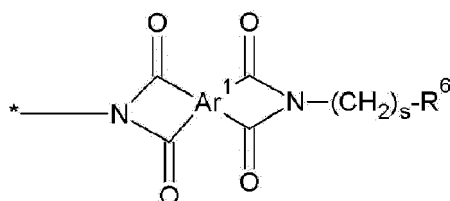
Chemical Formula 10
