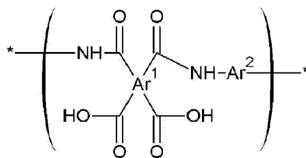
Chemical Formula 3
