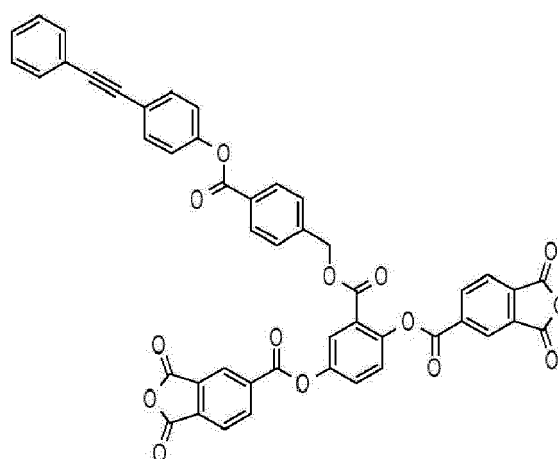
Compound M-6
