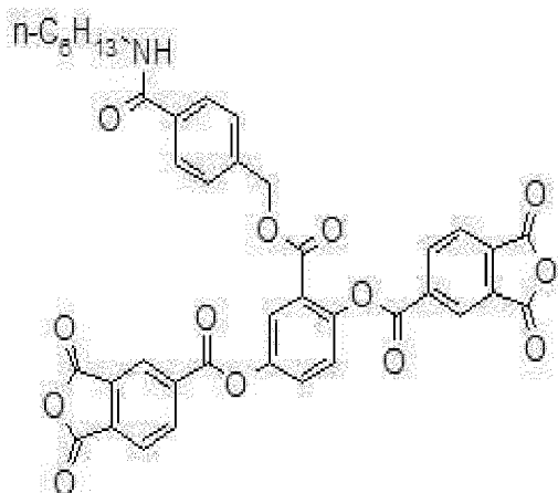
Compound M-14
