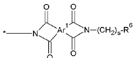
Chemical Formula 10
