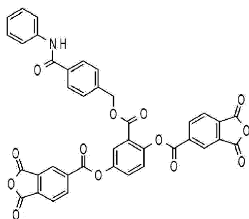
Compound M-5
