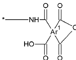
Chemical Formula 8
