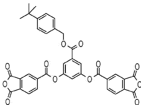
Compound M-9
