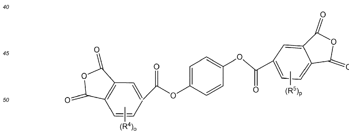
Chemical Formula 14-3
