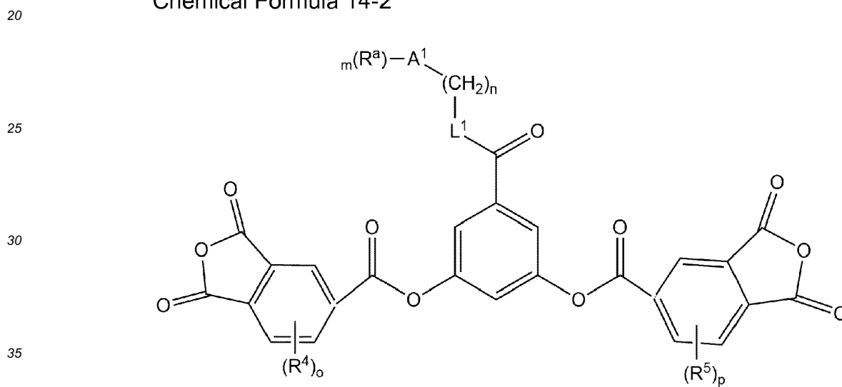
Chemical Formula 14-3
