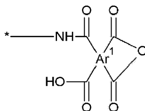
Chemical Formula 8
