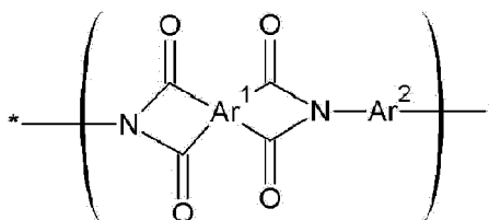
Chemical Formula 7
