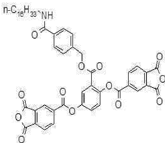
Compound M-16
