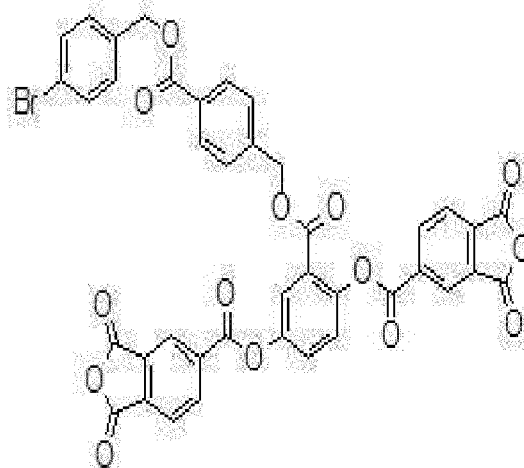
Compound M-15
