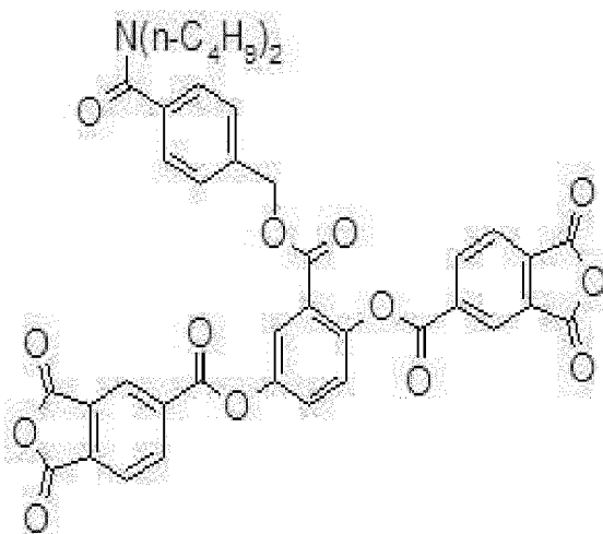
Compound M-18
