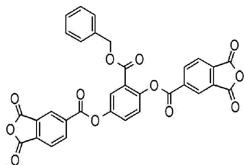
Compound M-3
