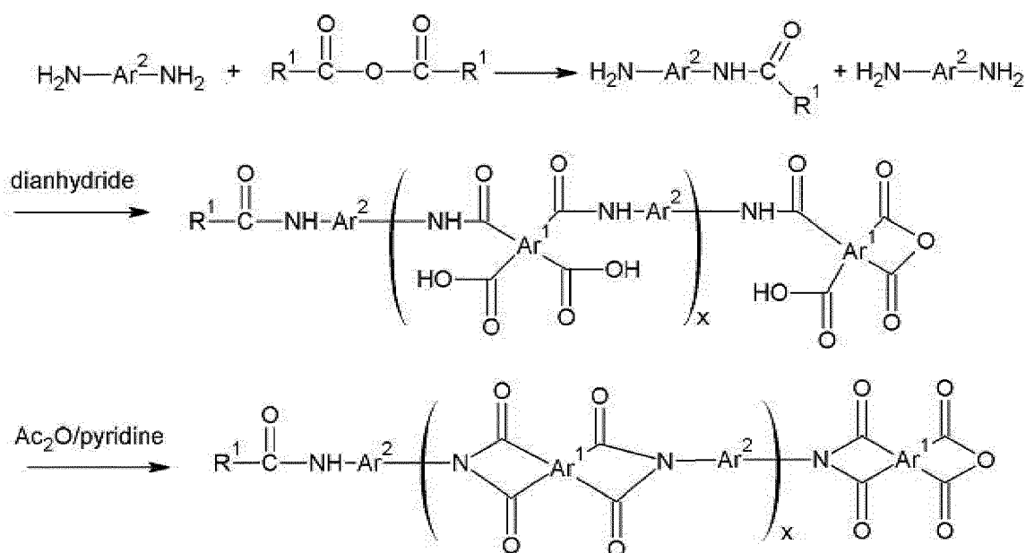
Reaction Scheme 1
