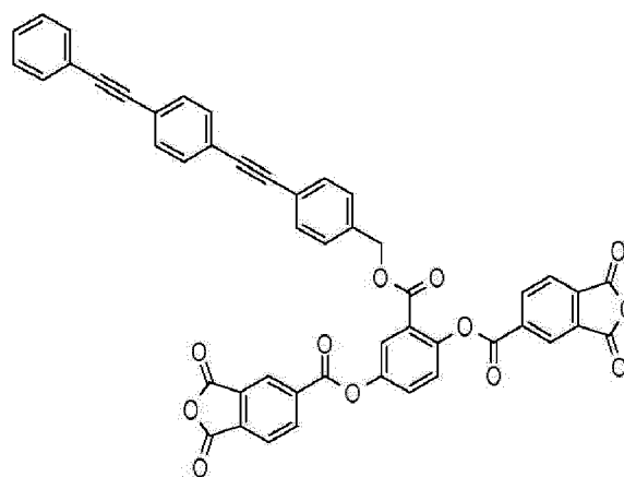
Compound M-6
