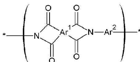
Chemical Formula 3
