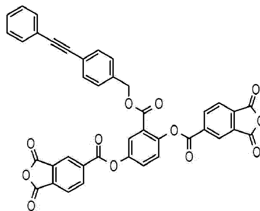
Compound M-2
