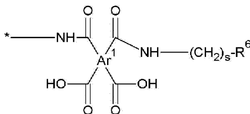
Chemical Formula 10
