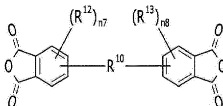
Chemical Formula 13
