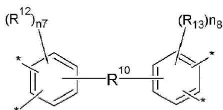
Chemical Formula 4
