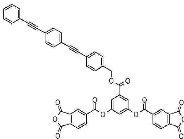
Compound M-9
