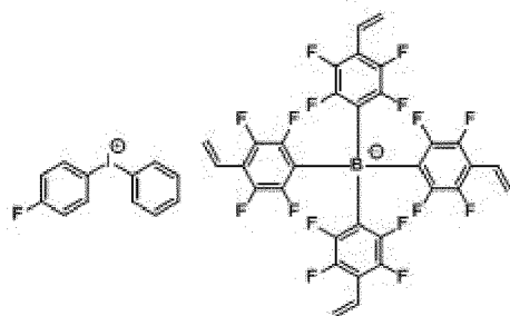
[Chemical Formula 1-1-9]
