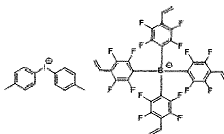
[Chemical Formula 1-1-4]
