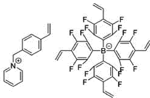
[Compound 6]
