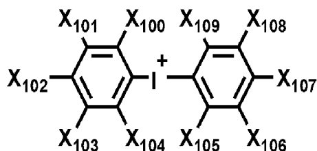
[Chemical Formula 11]
