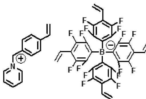
[Chemical Formula 1-3-4]
