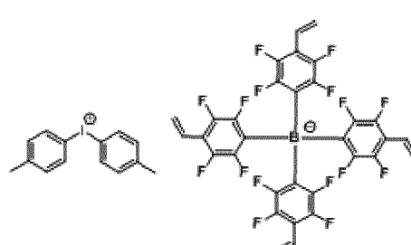
[Chemical Formula 1-1-4]
