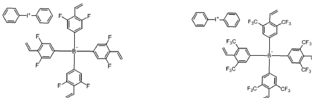
[Chemical Formula 1-1-24]
