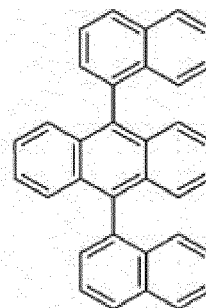
[Compound E]
