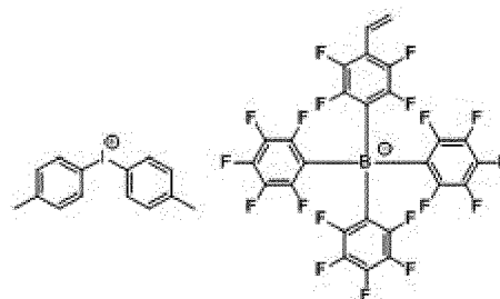
[Chemical Formula 1-1-17]
