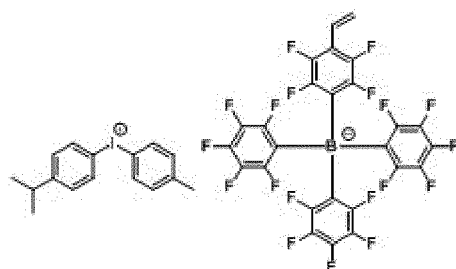
[Chemical Formula 1-1-14]
