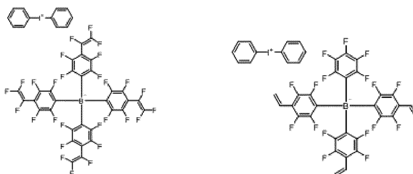
[Chemical Formula 1-1-21]
