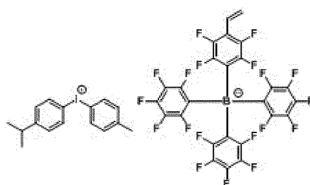
[Chemical Formula 1-1-14]
