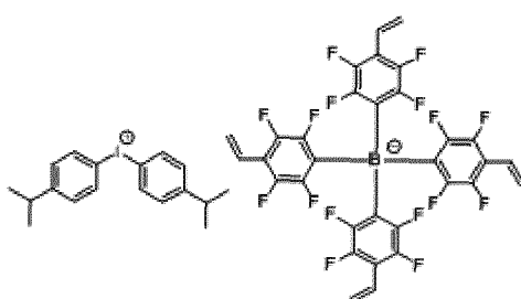
[Chemical Formula 1-1-3]
