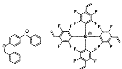
[Chemical Formula 1-1-7]
