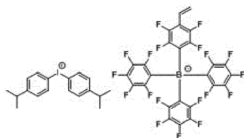
[Chemical Formula 1-1-16]
