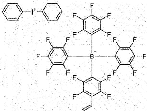
[Compound 9]
