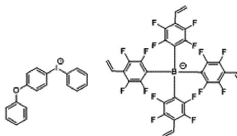
[Chemical Formula 1-1-8]
