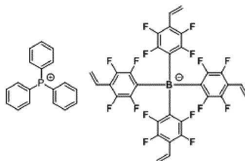
[Chemical Formula 1-2-2]
