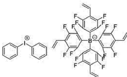
[Compound 9]
