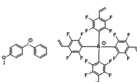
[Chemical Formula 1-1-6]
