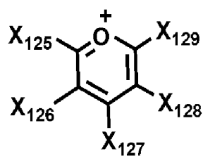
[Chemical Formula 13]
