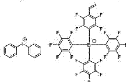
[Chemical Formula 1-1-15]
