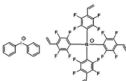
[Chemical Formula 1-1-2]
