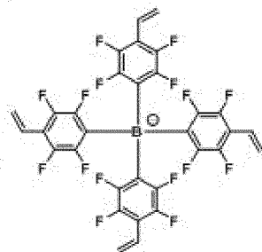
[Chemical Formula 1-1-10]
