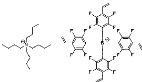
[Chemical Formula 1-3-3]
