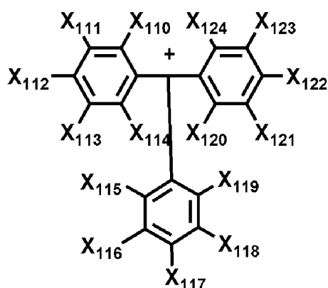
[Chemical Formula 12]
