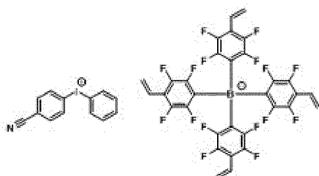
[Chemical Formula 1-1-14]
