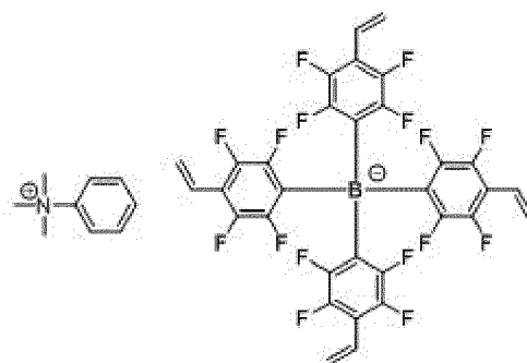
[Chemical Formula 1-3-2]
