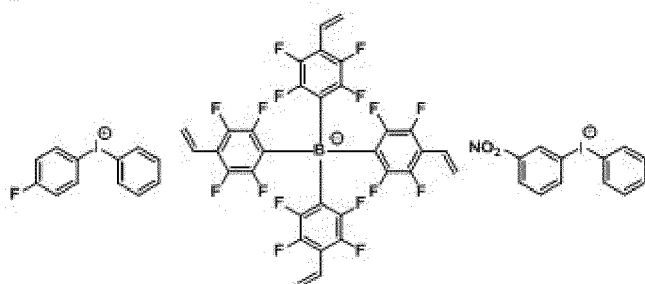
[Chemical Formula 1-1-9]
