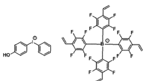
[Chemical Formula 1-1-5]
