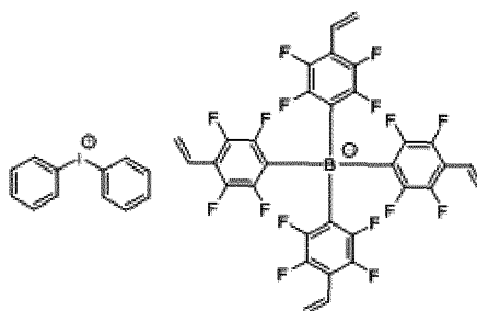
[Chemical Formula 1-1-2]
