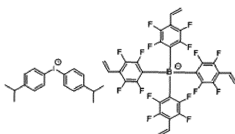
[Chemical Formula 1-1-3]
