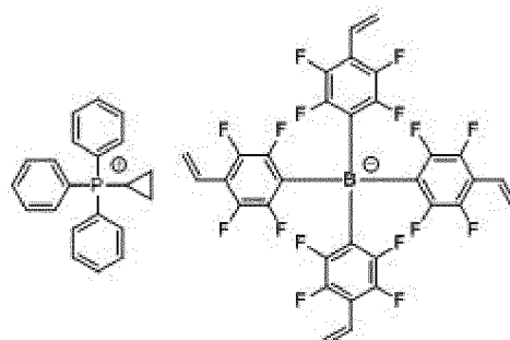
[Chemical Formula 1-2-5]
