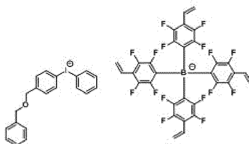
[Chemical Formula 1-1-12]
