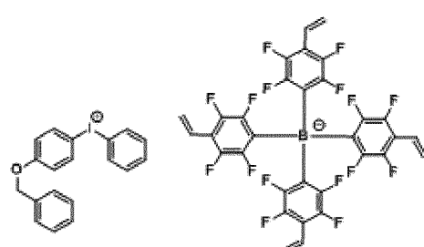
[Chemical Formula 1-1-7]
