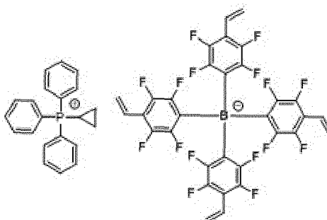
[Chemical Formula 1-2-5]
