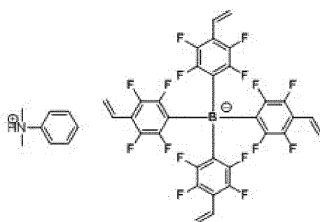
[Chemical Formula 1-3-1]
