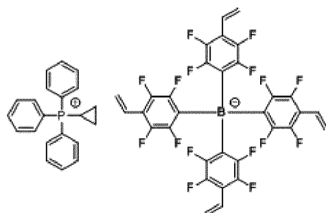
[Chemical Formula 1-5-1]
