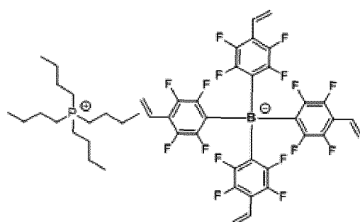
[Chemical Formula 1-2-1]
