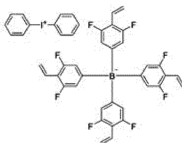
[Compound 4]
