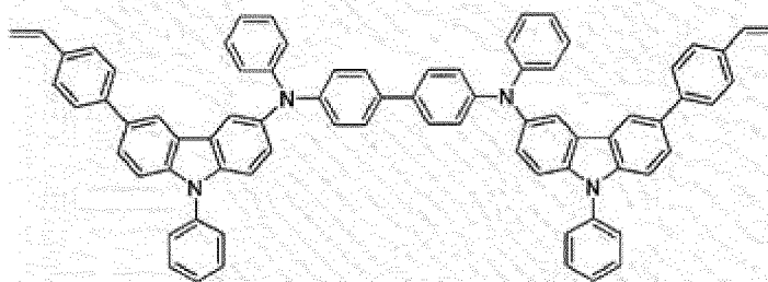
[Compound A]
