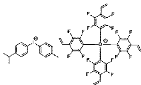
[Chemical Formula 1-1-1]
