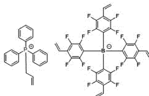
[Chemical Formula 1-2-4]
