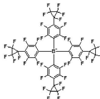
[Chemical Formula 1-2-2]
