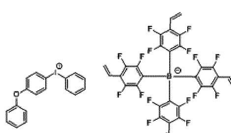
[Chemical Formula 1-1-8]
