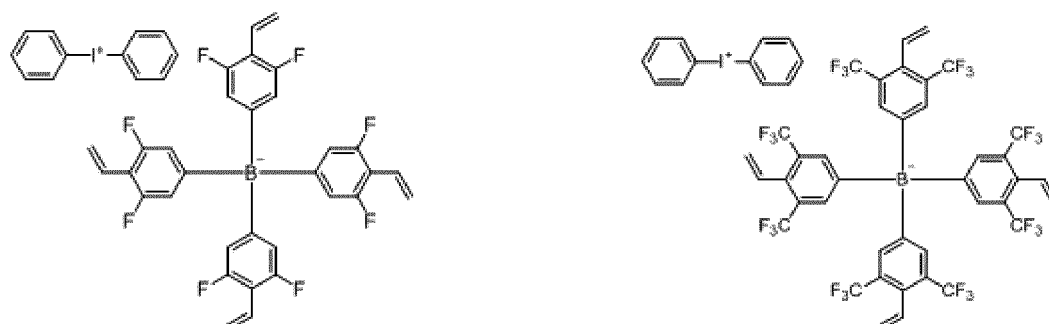
[Chemical Formula 1-1-23]
