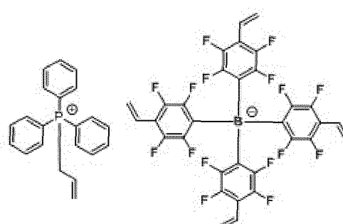
[Chemical Formula 1-2-4]
