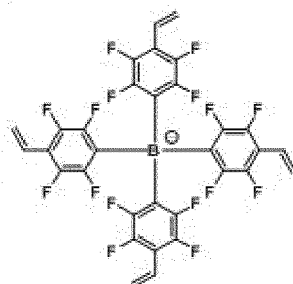
[Chemical Formula 1-1-10]
