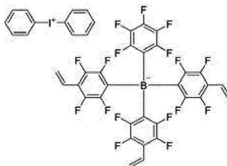
[Compound 3]
