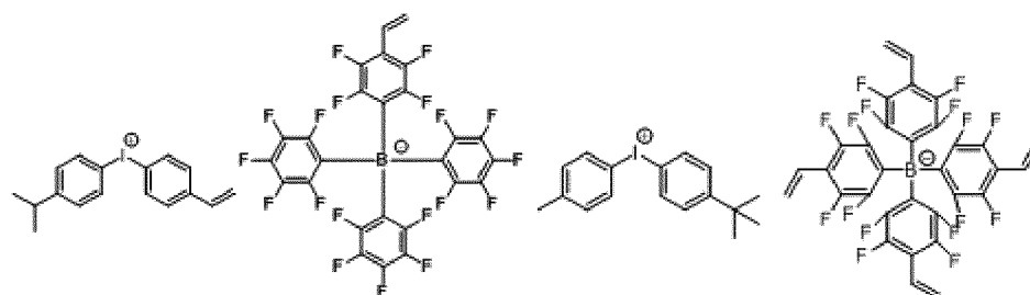
[Chemical Formula 1-1-20]
