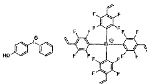
[Chemical Formula 1-1-5]
