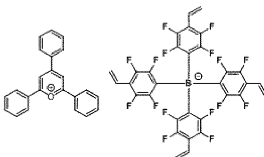
[Chemical Formula 1-4-1]
