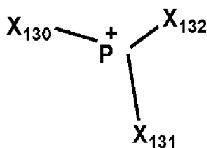
[Chemical Formula 13]
