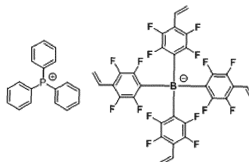
[Chemical Formula 1-2-2]
