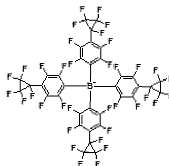
[Chemical Formula 1-2-2]
