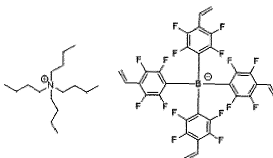
[Chemical Formula 1-3-3]
