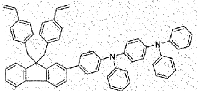
[Compound B]
