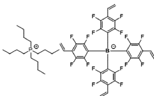
[Chemical Formula 1-2-1]
