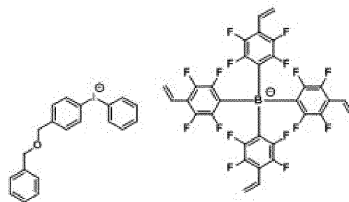
[Chemical Formula 1-1-12]
