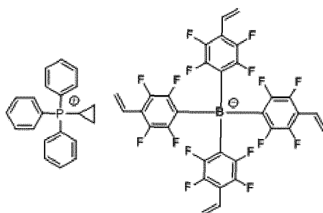
[Chemical Formula 1-5-1]
