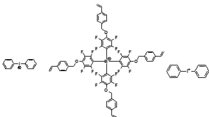
[Chemical Formula 1-1-25]
