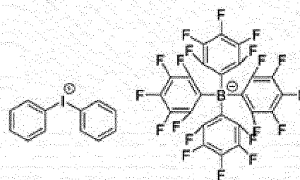
[Comparative Compound 2]
