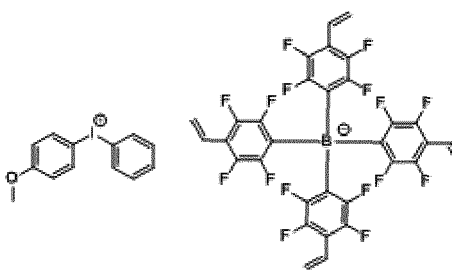
[Chemical Formula 1-1-6]
