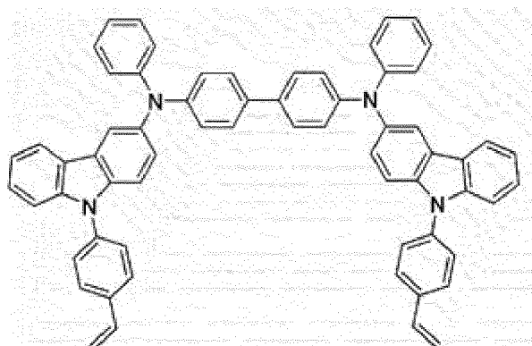
[Compound C]
