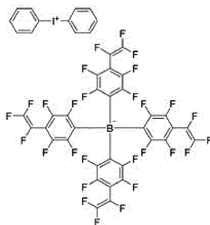
[Compound 2]
