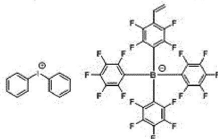
[Chemical Formula 1-1-15]
