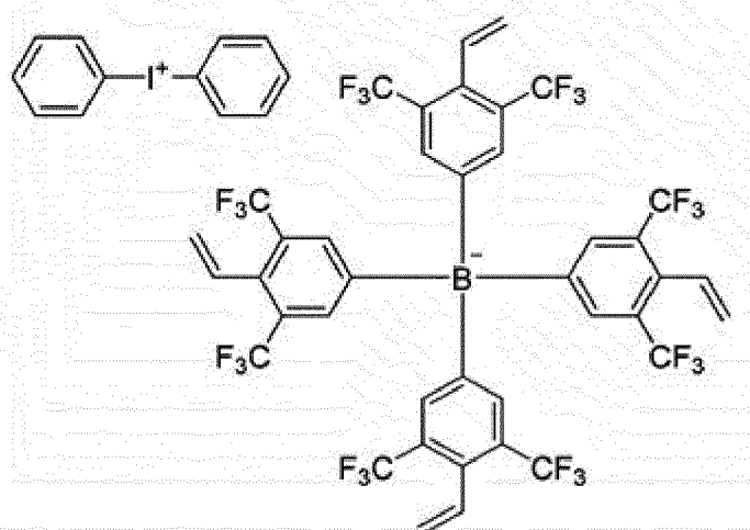
[Comparative Compound 1]
