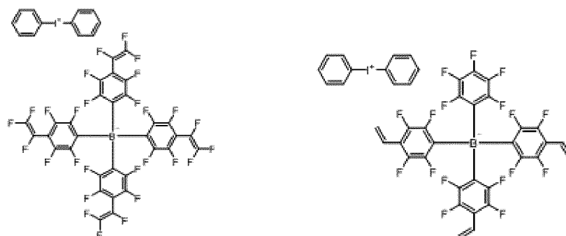
[Chemical Formula 1-1-21]
