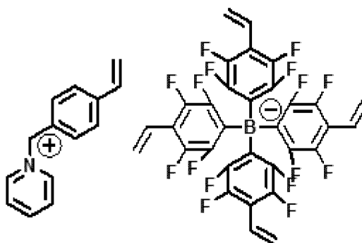
[Chemical Formula 1-3-4]
