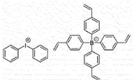
[Comparative Compound 1]
