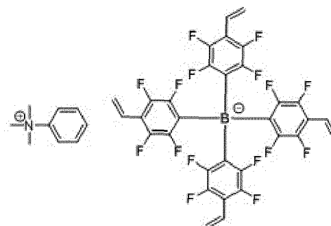
[Chemical Formula 1-3-2]
