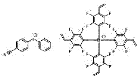
[Chemical Formula 1-1-14]
