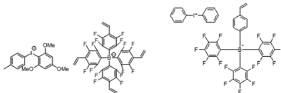
[Chemical Formula 1-1-20]
