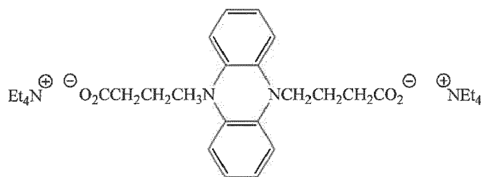
phenazine 3
