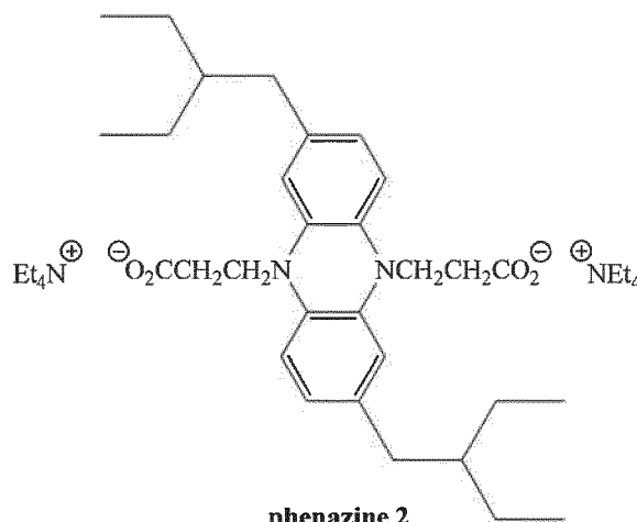
phenazine 2
