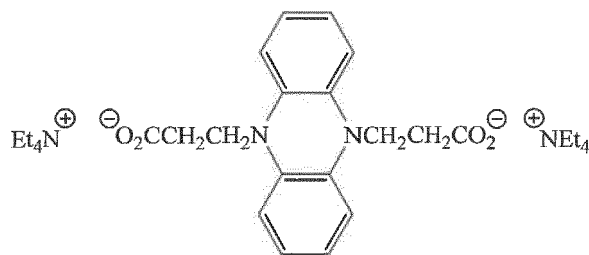
phenazine 1
