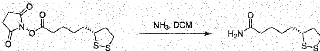
Scheme 2. Synthetic scheme for (R)-lipoamide.
