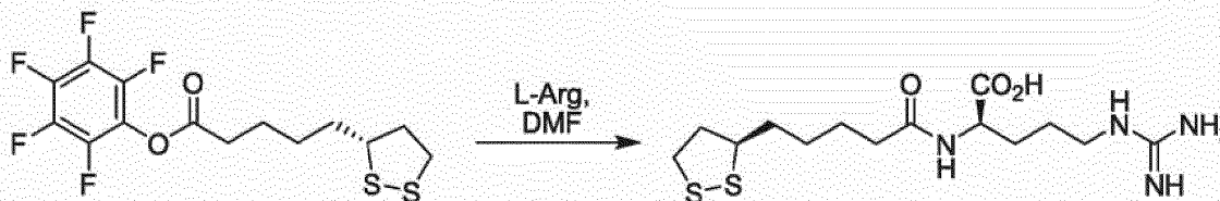
Scheme 4. Synthetic scheme for LA-Arg.
