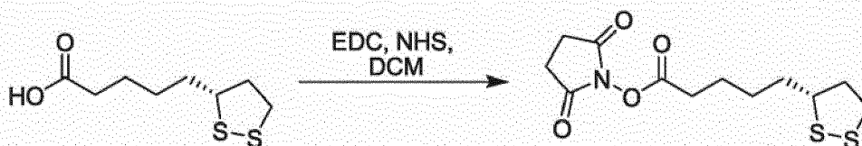
Scheme 1. Synthetic scheme for NHS-ester of (R)-lipoic acid.
