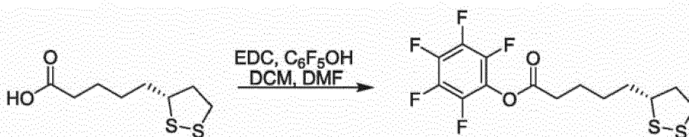
Scheme 3. Synthetic scheme for pentafluorophenyl ester of (R)-lipoic acid.
