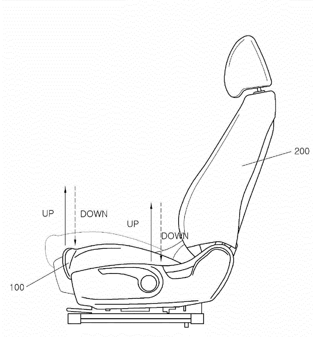
FIG.14 (RELATED ART)
