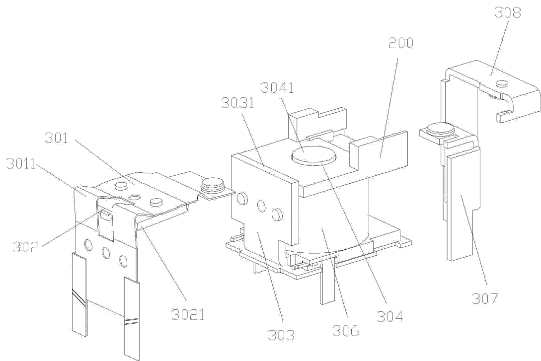
Fig.12 (Prior Art )
