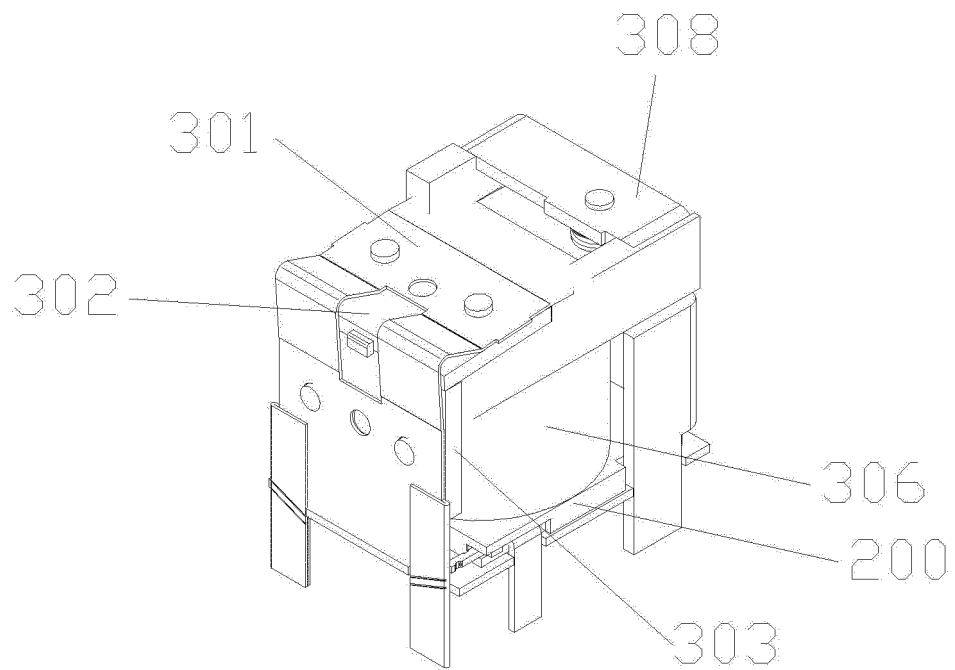
Fig.11 (Prior Art)
