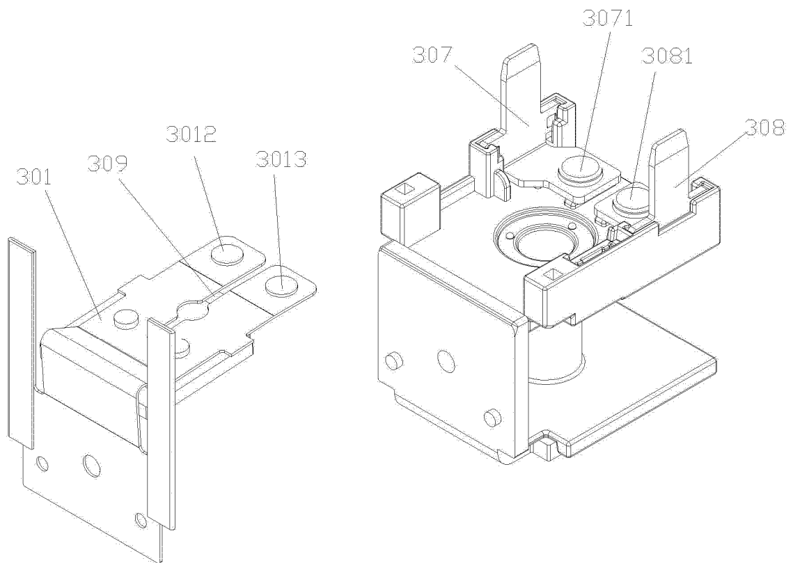
Fig.26 (Prior Art )
