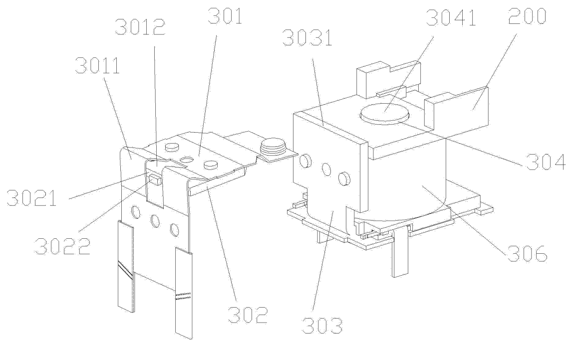
Fig.18 (Prior Art)
