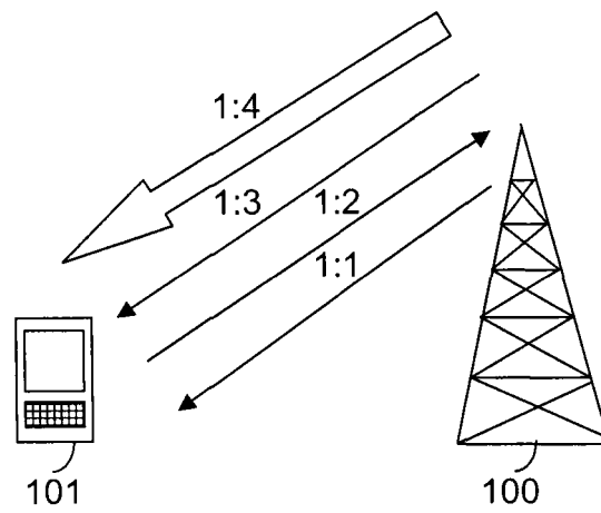
Figure 1 (PRIOR ART)
