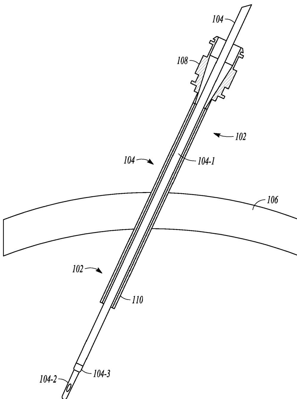
FIG. 1 (PRIOR ART)
