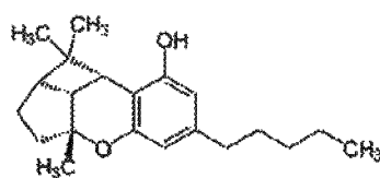
Cannabicyclol (CBL)
