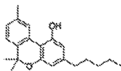
Cannabinol CBN-C 5
