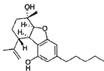
Cannabielsoin-type (CBE)
