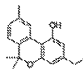
Cannabinol-C 2 CBN-C 2
