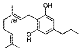
Cannabigerovarin (CBGV)
