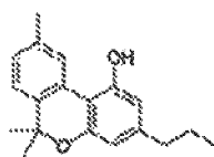
Cannabivarin CBN-C 3
