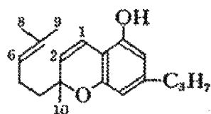
CBCV (Cannabichromevarin)
