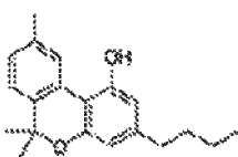
Cannabinol-C 4 CBN-C 4
