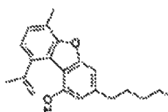
Dehydrocannabifuran DCBF-C 5
