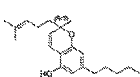
(±)-Cannabichromene CBC-C 5
