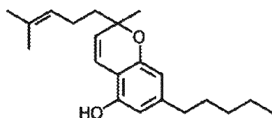
Cannabichromene (CBC)
