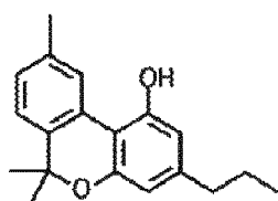
Cannabivarin (CBV)
