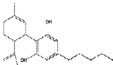
Cannabidiol (CBD)
