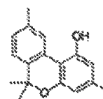
Cannabiorcol CBN-C 1
