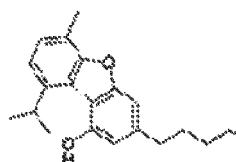
Cannabifuran CBF-C 5
