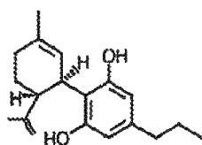
Cannabidivarin (CBDV)
