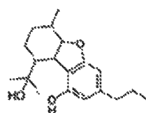
Cannabiglendol-C 3 OH-iso-HHCV-C 3
