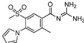
Eniporide
