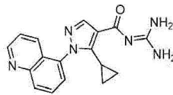
Zoniporide
