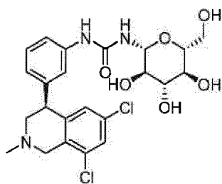
SAR218034
