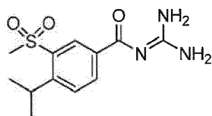
Cariporide
