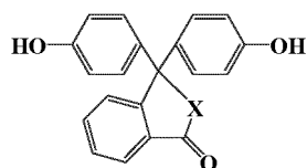
[Chemical formula 2-1]
