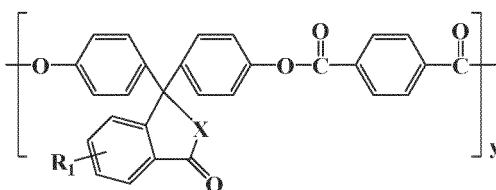
[Chemical formula 1]
