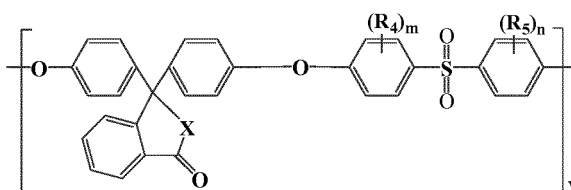
[Chemical formula 2]
