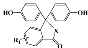
[Chemical formula 1-2]
