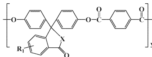
[Chemical formula 1]
