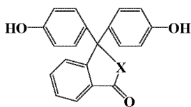
[Chemical formula 2-1]
