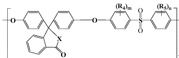
[Chemical formula 2]
