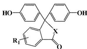
[Chemical formula 1-2]
