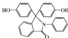
[Chemical formula 9-1]
