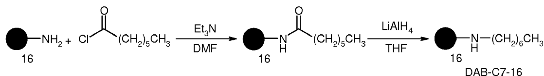
Scheme 4. Preparation of DAB-C7-16.
