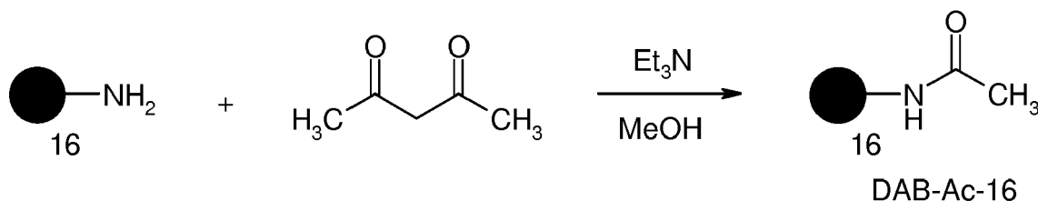
Scheme 6. Preparation of DAB-Ac-16.
