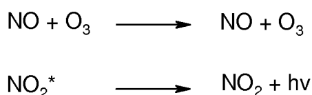
Scheme 2. Measurement of NO by chemiluminescence.
