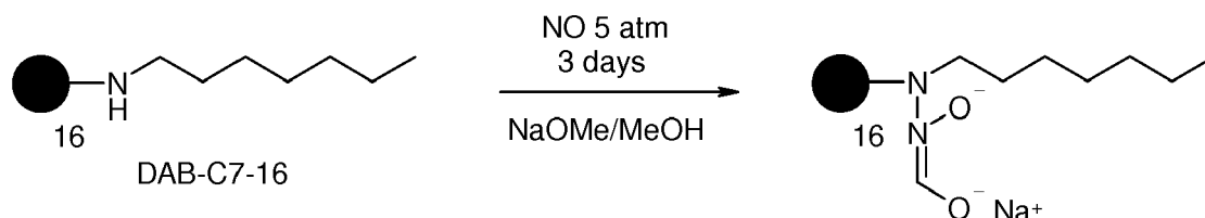
Scheme 5. Preparation of DAB-C7-16 diazeniumdiolate.
