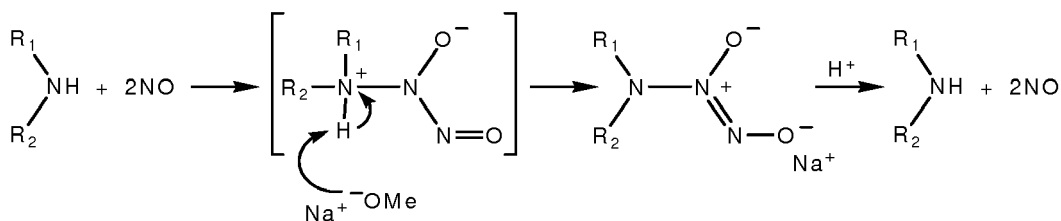
Scheme 1. Synthesis and NO-release from N-diazeniumdiolates.
