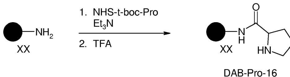
Scheme 7. Preparation of DAB-Pro-16.
