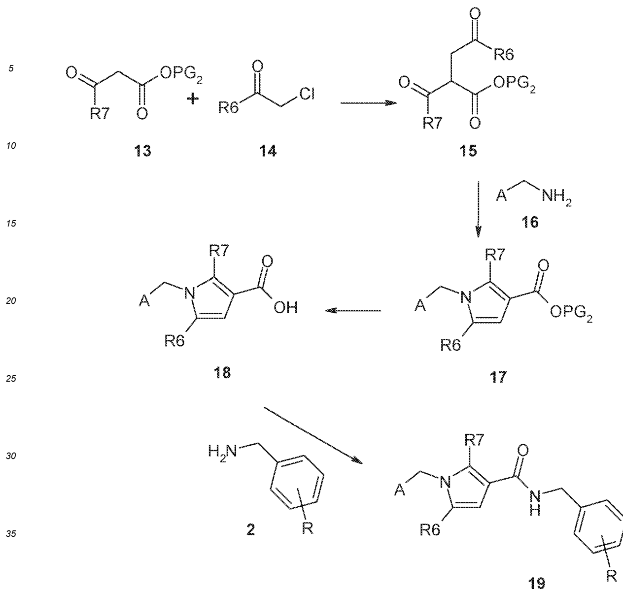
Scheme 3
