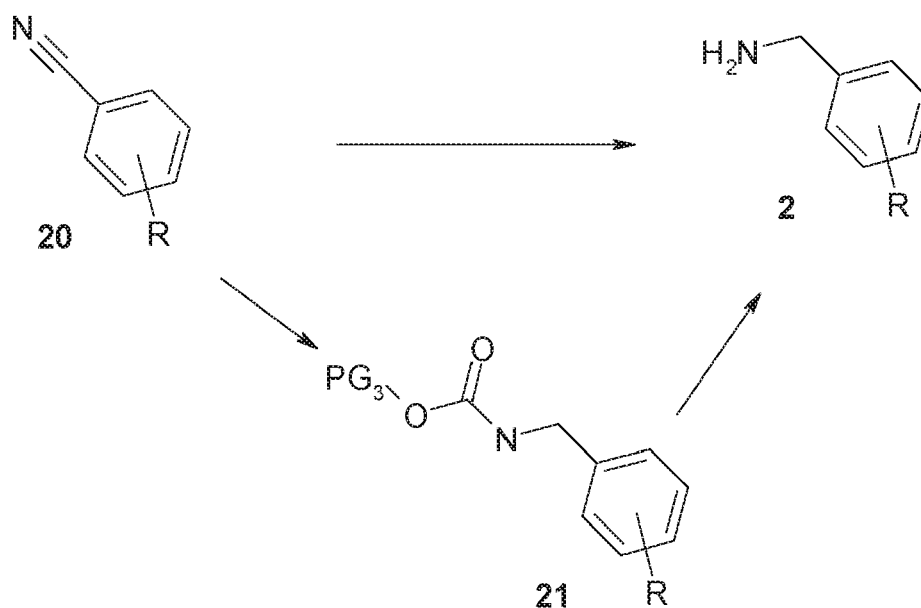
Scheme 4
