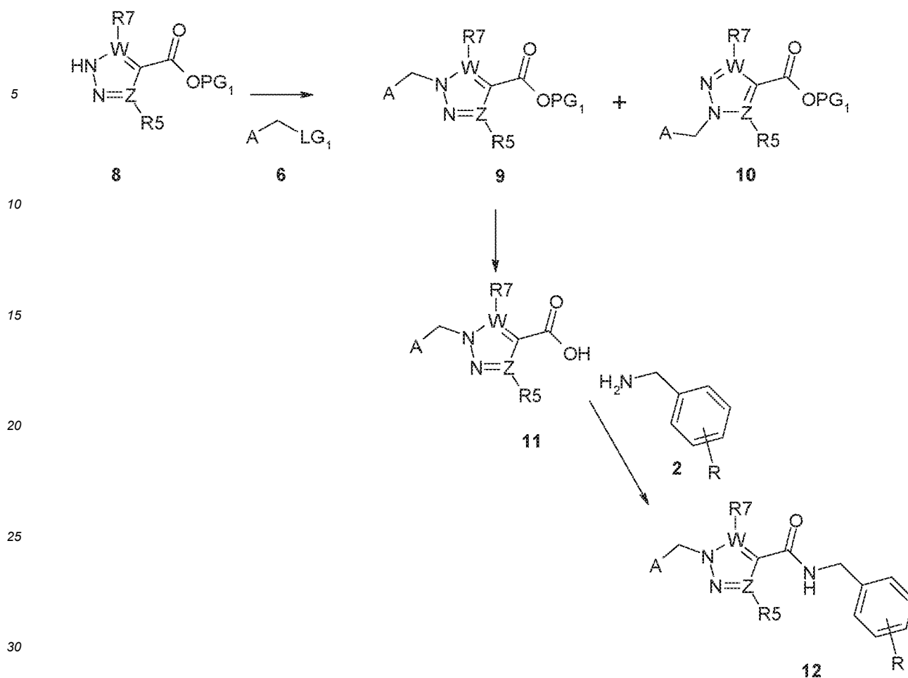
Scheme 2b
