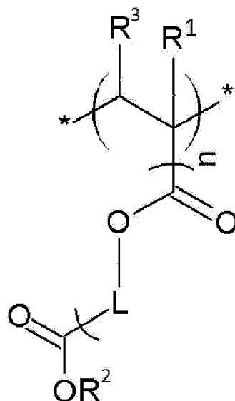
Chemical Formula 4
