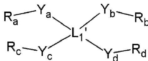
Chemical Formula 6-1
