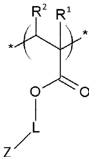
Chemical Formula 3
