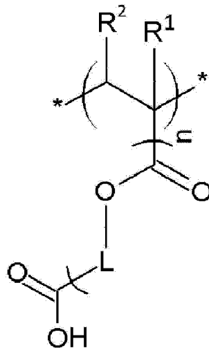
Chemical Formula 1-2
