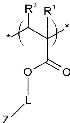
Chemical Formula 3
