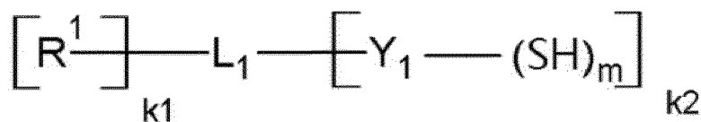
Chemical Formula 6
