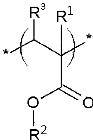
Chemical Formula 2
