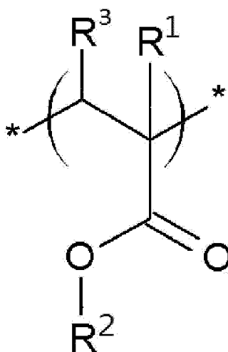
Chemical Formula 2
