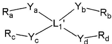
Chemical Formula 6-1
