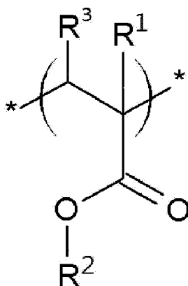
Chemical Formula 2
