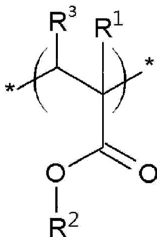
Chemical Formula 2
