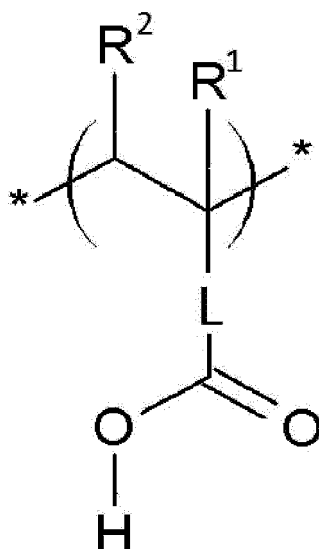
Chemical Formula 1-1
