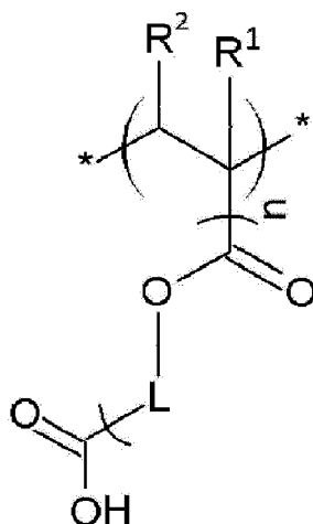
Chemical Formula 1-2
