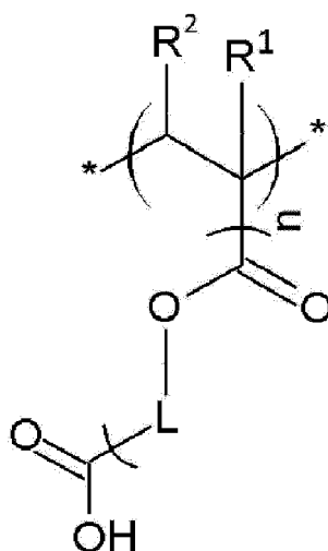
Chemical Formula 1-2
