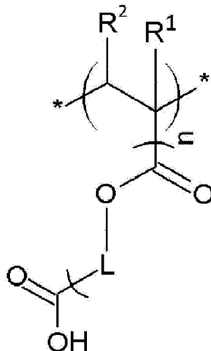
Chemical Formula 1-2
