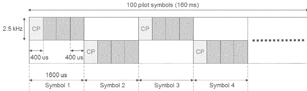
Figure 5A: PRACH Format 2
