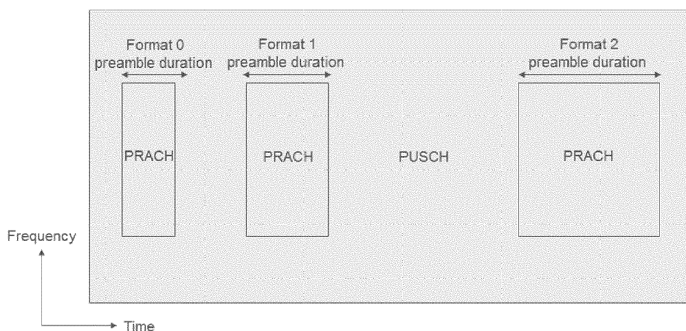
Figure 2A: Multiplexing of Uplink Physical Channels
