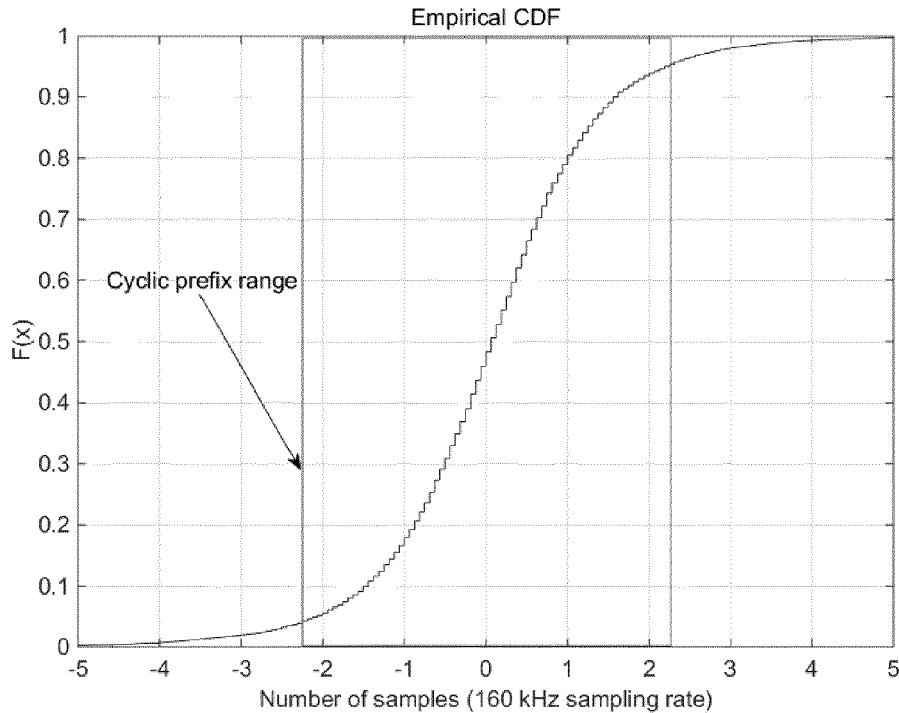
Figure 8A: Distribution of time-of-arrival estimation errors: Format 2 at -4 dB SNR.
