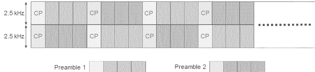
Figure 6A: Frequency multiplexing of preambles of Format 2
