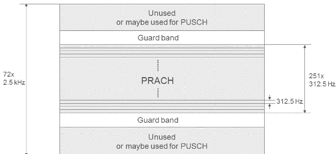
Figure 3A: Preamble length and subcarrier spacing for PRACH Formats 0 and 1
