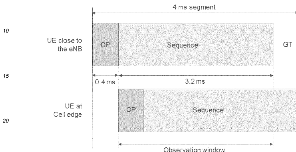
Figure 4A: Cyclic prefix/guard period dimensioning for PRACH Formats 0 and 1
