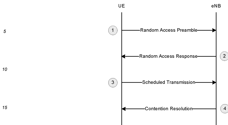
Figure 1A: LTE contention-based random access procedure [7]
