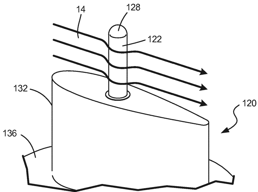
FIG. 3 (PRIOR ART)
