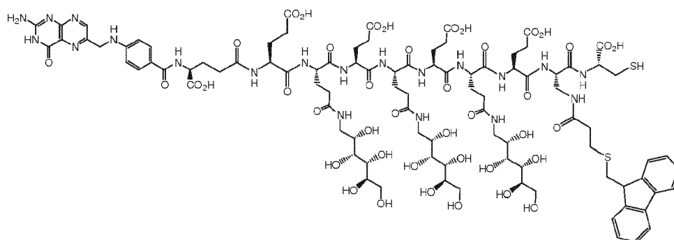
EC0682 Optionally selective multidrug intermediate for two drugs. C 95 H 132 N 20 O 42 S 2 , MW 2290.30, Exact Mass: 2288.82
