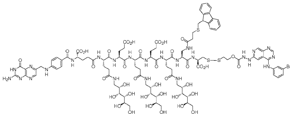
EC0679 Conjugate of 4-[(3-Bromophenyl)amino]-6-hydrazino-pyrido[3,4-d]pyrimidine and intermediate for multidrug conjugate. C 101 H 131 BrN 24 O 38 S 3 , MW 2465.36, Exact Mass: 2462.74
