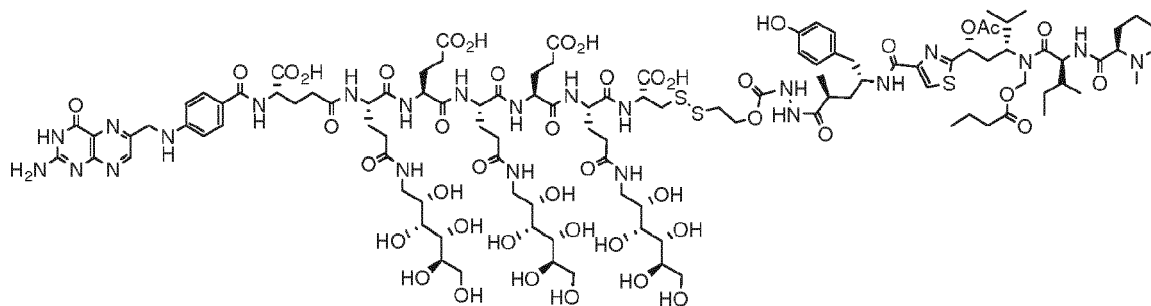
EC0531 Conjugate of Tubulysin
