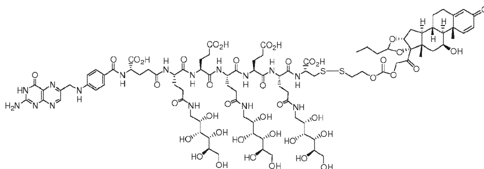
EC0600 Conjugate of Budesonide. C 93 H 134 N 16 O 42 S 2 , C, 50.49; H, 6.11; N, 10.13; O, 30.37; S, 2.90, MW 2212.27, Exact Mass: 2210.83
