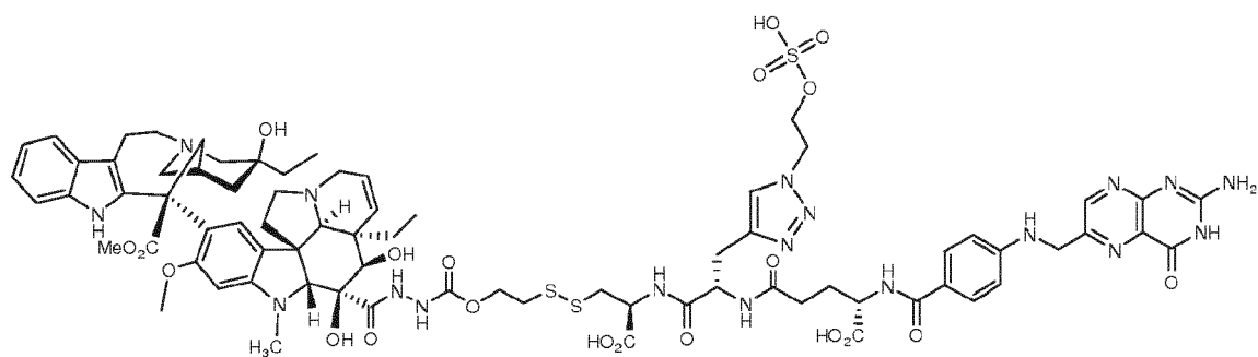
EC0418 Conjugate of DAVLBH
