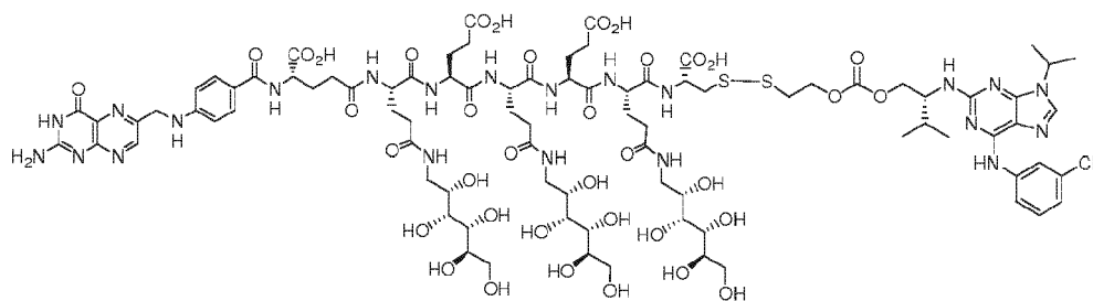
EC0545 Conjugate of purvalanol A. C 87 H 125 C 1 N 22 O 37 S 2 ; MW 2170.63, Exact Mass: 2168.77
