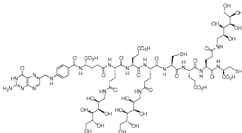
EC0593 Multidrug intermediate for two drugs. C 68 H 103 N 17 O 35 S 2 , MW 1782.77, Exact Mass: 1781.62
