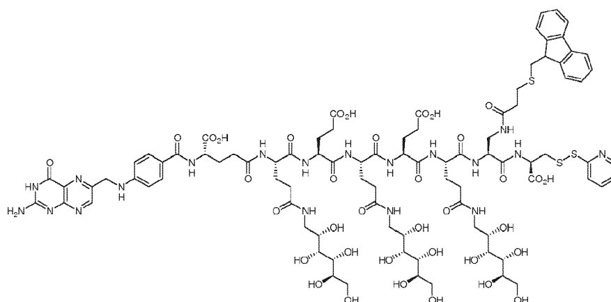
EC0559 Optionally selective multidrug intermediate for two drugs. C 90 H 121 N 19 O 36 S 3 , MW 2141.22, Exact Mass: 2139.74
