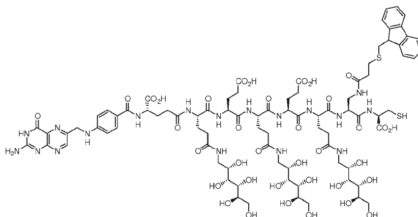
EC0542 Optionally selective multidrug intermediate for two drugs. C 85 H 118 N 18 O 36 S 2 , C, 50.24; H, 5.85; N, 12.41; O, 28.34; S, 3.16, MW 2032.08, Exact Mass: 2030.74
