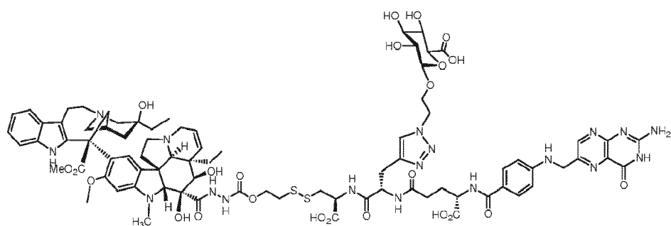
EC0400 Conjugate of DAVLBH. Prepared by Huisgen cyclization of corresponding alkyne and azidoethylcarbohydrate; 2 eq. Na ascorbate, 1 eq. CuSO 4 ·5H 2 O, THF/water (1:1); 5 eq. Na aAscorbate, 2.5 eq. CuSO 4 ·5H 2 O, THF/water (9:1); (10 mg). C 81 H 100 N 18 O 24 S 2 , C, 54.84; H, 5.68; N, 14.21; O, 21.65; S, 3.62, MW 1773.90, Exact Mass: 1772.66
