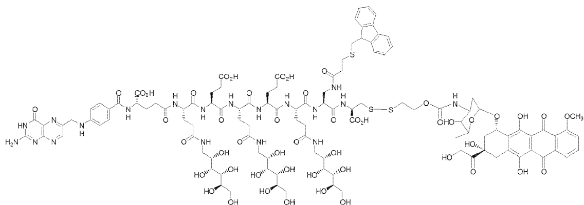
EC0693 Conjugate of Doxorubicin and intermediate for multidrug conjugate. C 115 H 149 N 19 O 49 S 3 , MW 2677.71, Exact Mass: 2675.89
