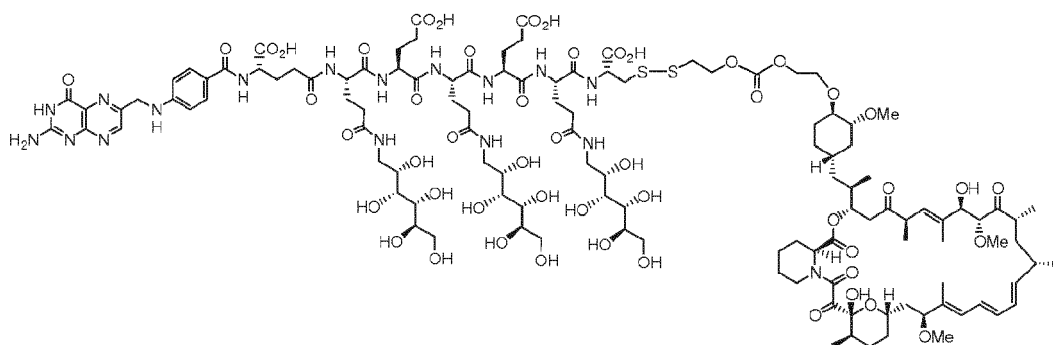
EC0565 Conjugate of everolimus. C 121 H 183 N 17 O 50 S 2 , MW 2739.96, Exact Mass: 2738.17
