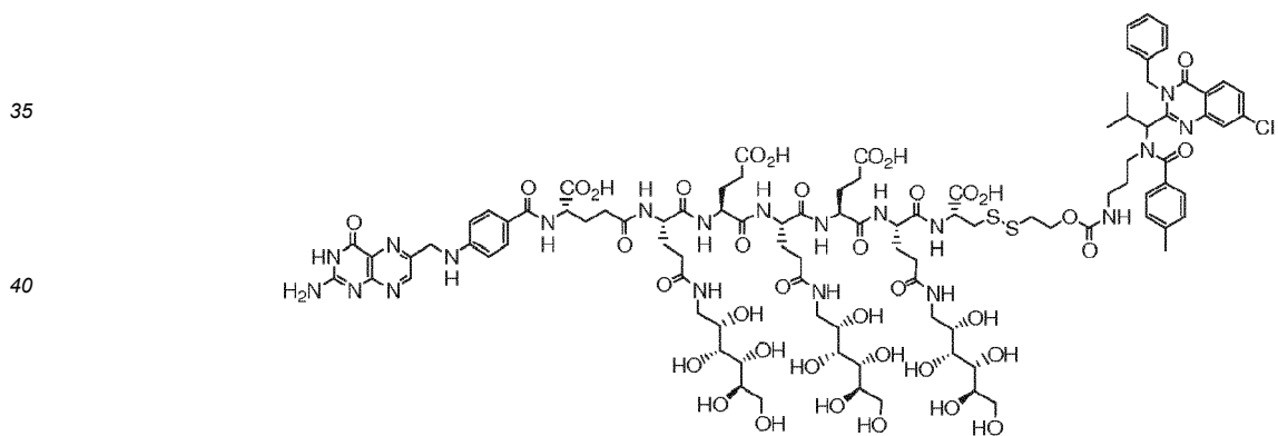
EC0581 Conjugate of ispinesib. C98H133C1N20O38S2, MW 2298.80, Exact Mass: 2296.82
