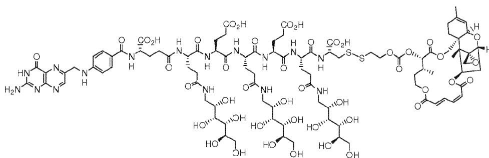
EC0598 Conjugate of Verucarin. C 95 H 134 N 16 O 45 S 2 , MW 2284.29, Exact Mass: 2282.81
