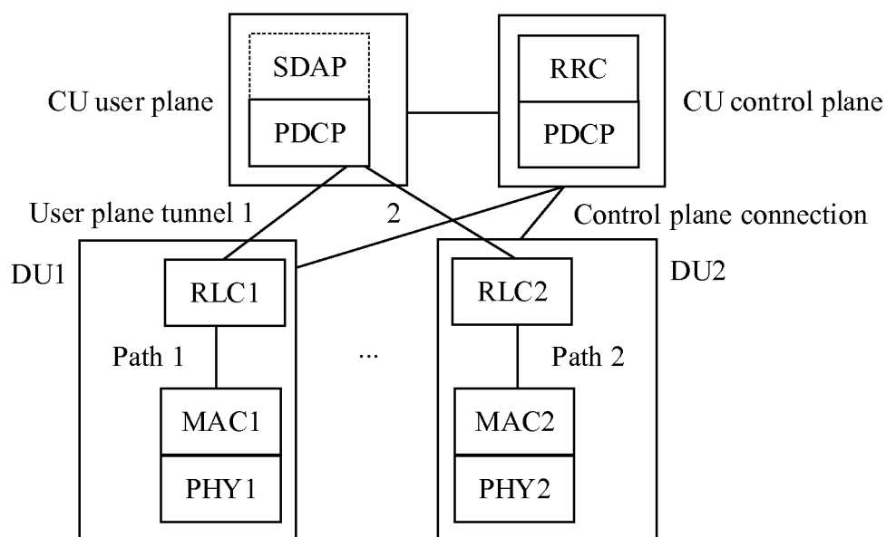
CU-DU architecture 2
