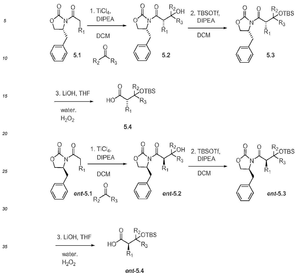
Scheme 5
