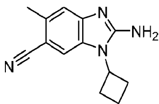
2-amino-1-(tert-butyl)-5-methyl-1H-benzo[d]imidazole-6-carbonitrile
