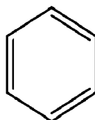
phenyl
