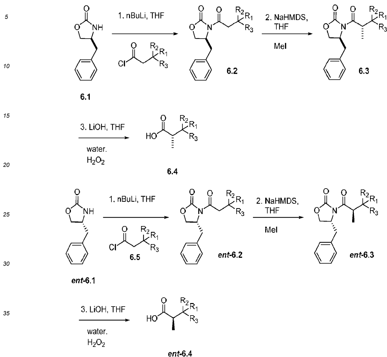
Scheme 6
