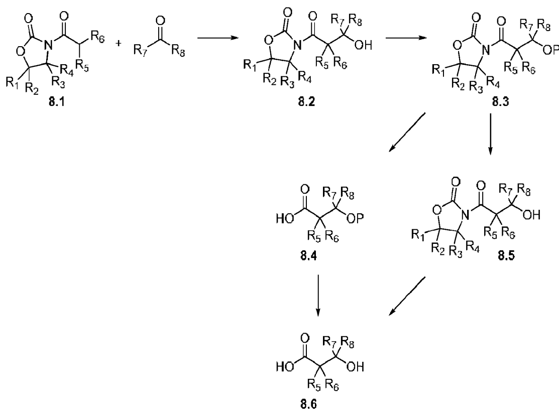
Scheme 8
