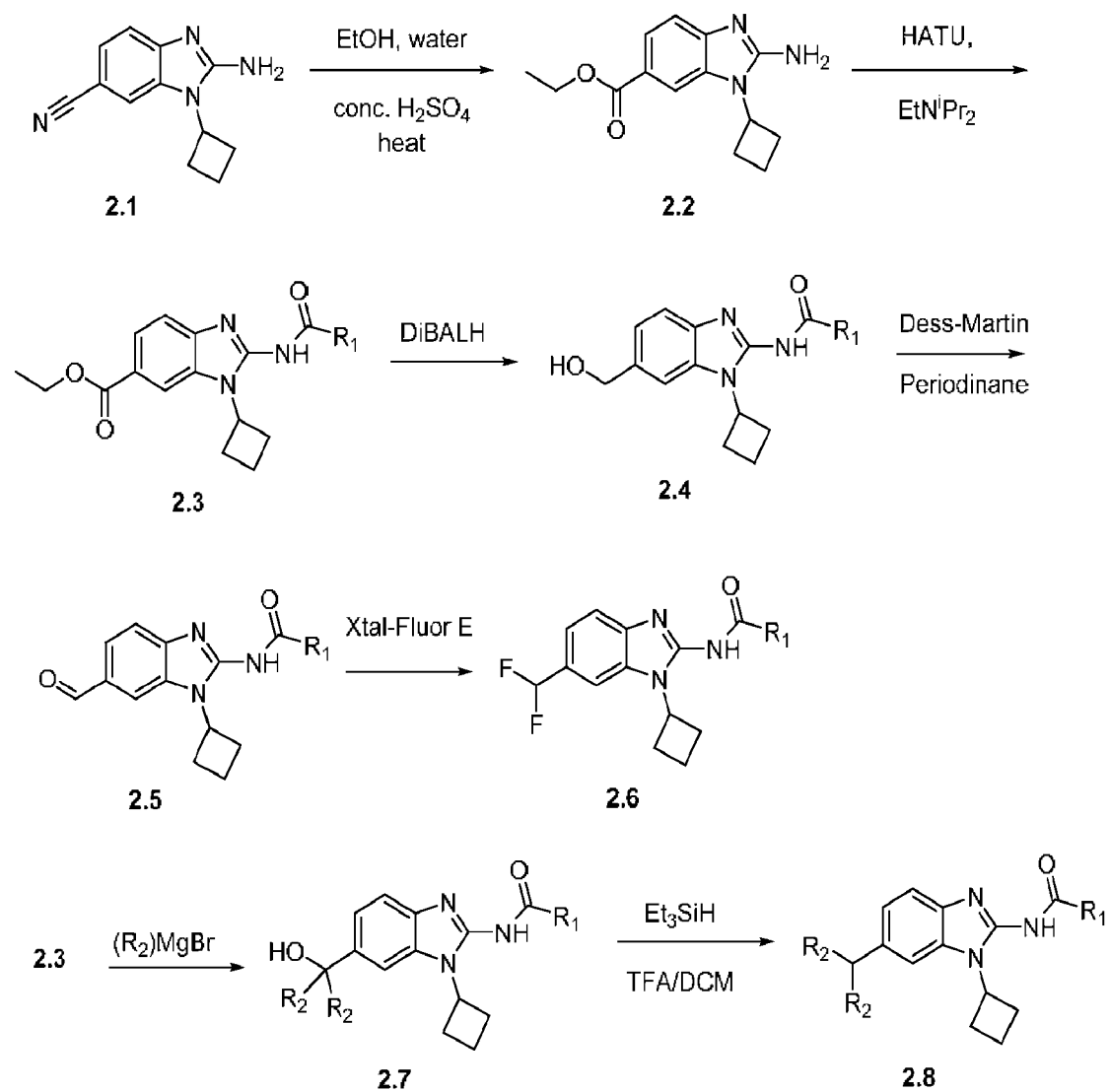
Scheme 3
