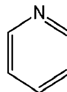
pyridinyl
