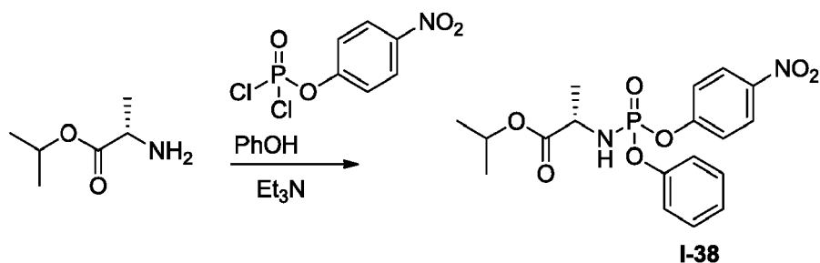
(2S)-Isopropyl 2-(((4-nitrophenoxy)(phenoxy)phosphoryl)amino)propanoate (I-38)
