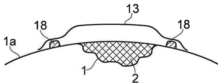
FIG. 3b/cross-section
