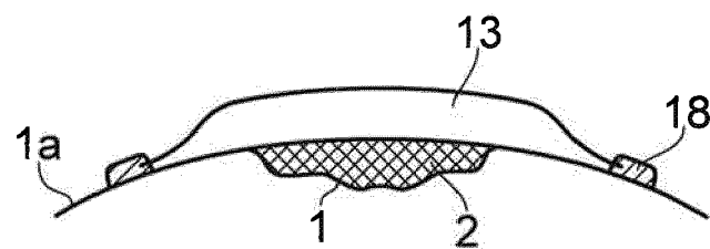
FIG. 2f/cross-section
