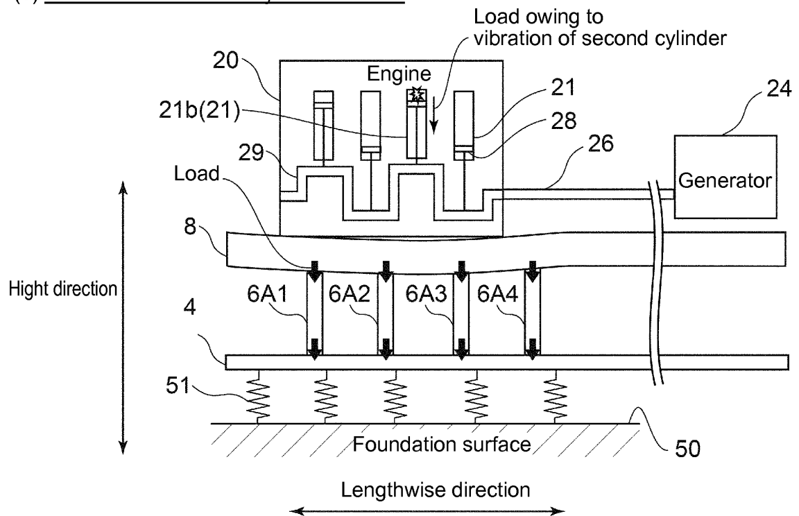
(b) Case in which second cylinder vibrates
