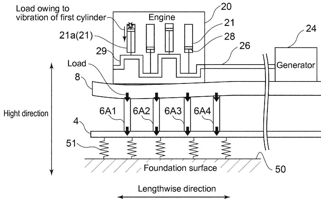
(a) Case in which first cylinder vibrates
